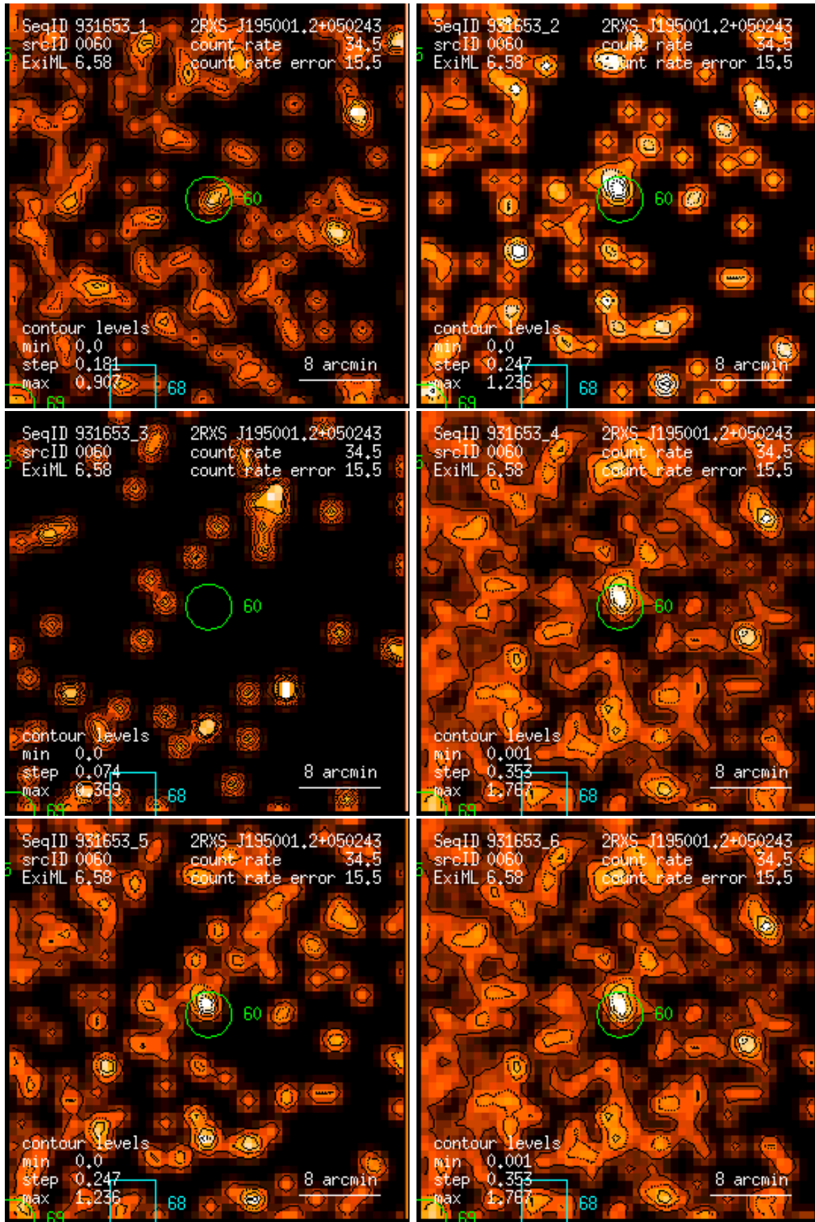
Figure 60: RASS 931653: detection 0060: band rate images, Gaussian filter: (1) PSPC channels 11 – 41, (2) 52 – 90, (3) 91 – 201, (4) 11 – 235, (5) 52 – 201, (6) 11 – 201. Broad band rates in counts/ks. Band rate contour levels in counts/ks/arcmin 2 .
