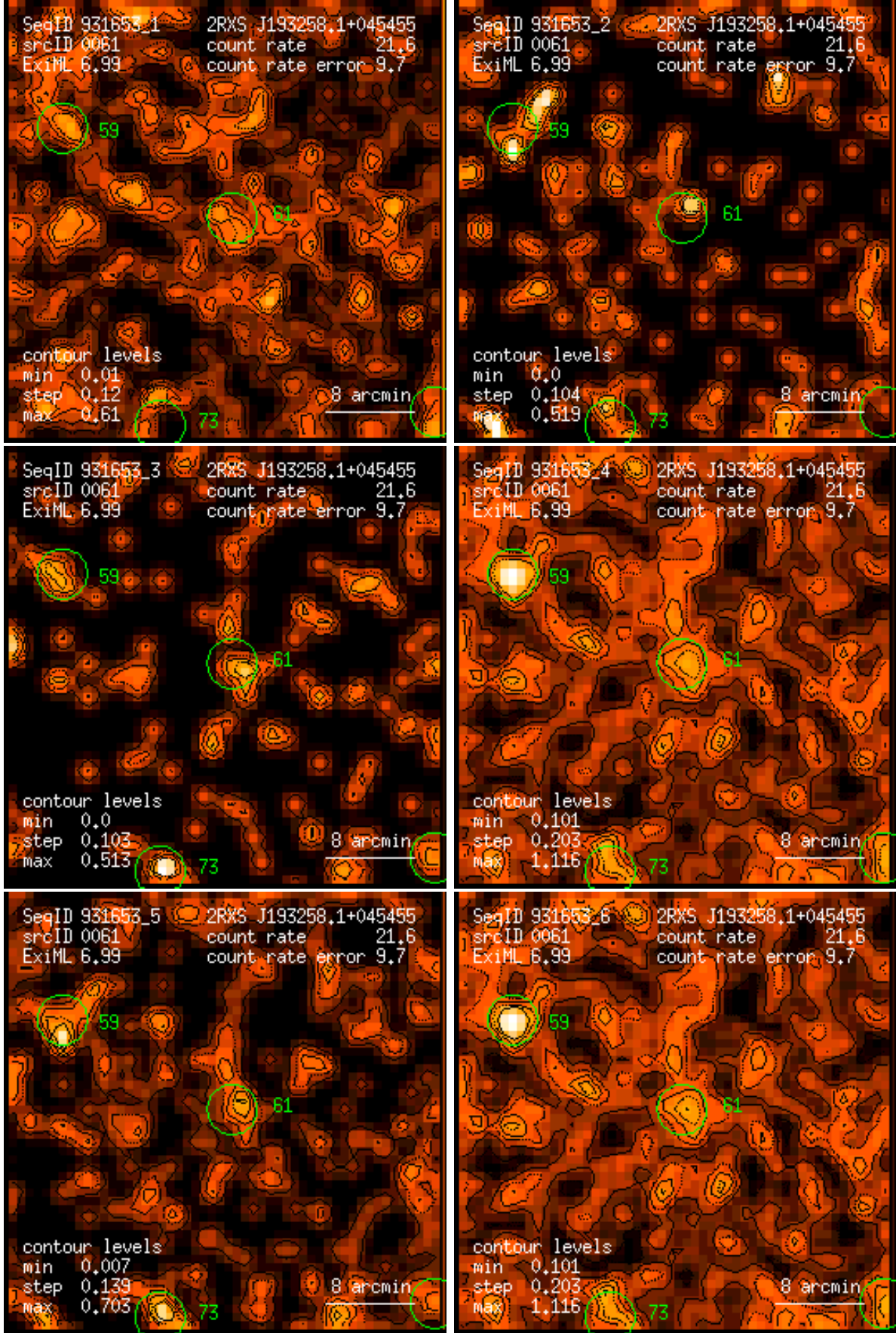
Figure 61: RASS 931653: detection 0061: band rate images, Gaussian filter: (1) PSPC channels 11 – 41, (2) 52 – 90, (3) 91 – 201, (4) 11 – 235, (5) 52 – 201, (6) 11 – 201. Broad band rates in counts/ks. Band rate contour levels in counts/ks/arcmin 2 .
