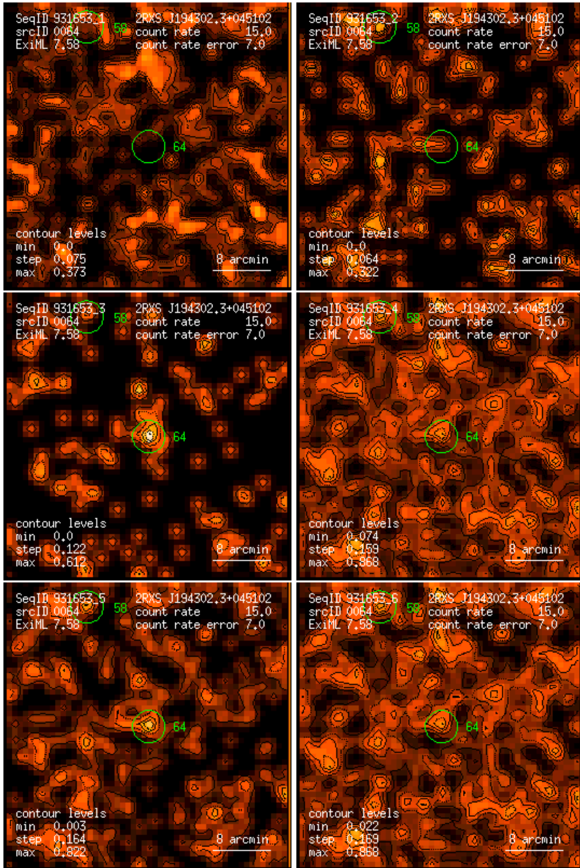
Figure 64: RASS 931653: detection 0064: band rate images, Gaussian filter: (1) PSPC channels 11 – 41, (2) 52 – 90, (3) 91 – 201, (4) 11 – 235, (5) 52 – 201, (6) 11 – 201. Broad band rates in counts/ks. Band rate contour levels in counts/ks/arcmin 2 .
