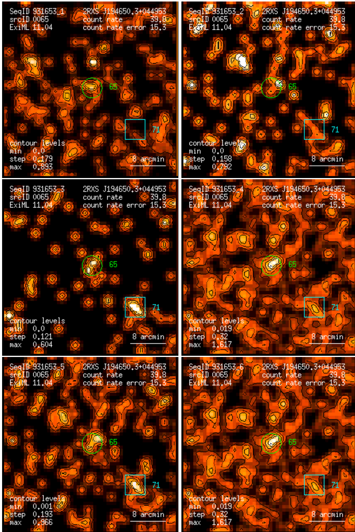
Figure 65: RASS 931653: detection 0065: band rate images, Gaussian filter: (1) PSPC channels 11 – 41, (2) 52 – 90, (3) 91 – 201, (4) 11 – 235, (5) 52 – 201, (6) 11 – 201. Broad band rates in counts/ks. Band rate contour levels in counts/ks/arcmin 2 .
