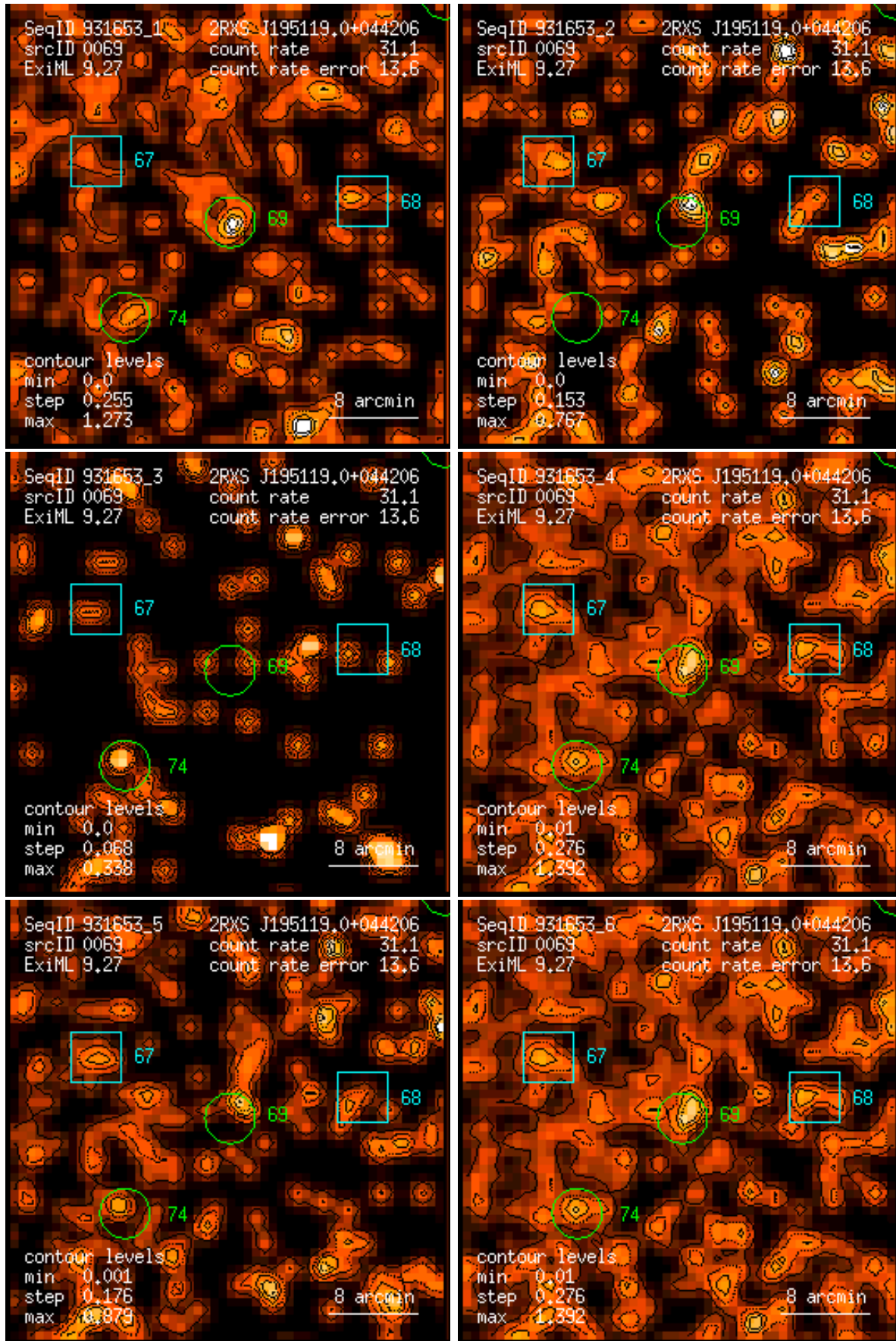
Figure 69: RASS 931653: detection 0069: band rate images, Gaussian filter: (1) PSPC channels 11 – 41, (2) 52 – 90, (3) 91 – 201, (4) 11 – 235, (5) 52 – 201, (6) 11 – 201. Broad band rates in counts/ks. Band rate contour levels in counts/ks/arcmin 2 .
