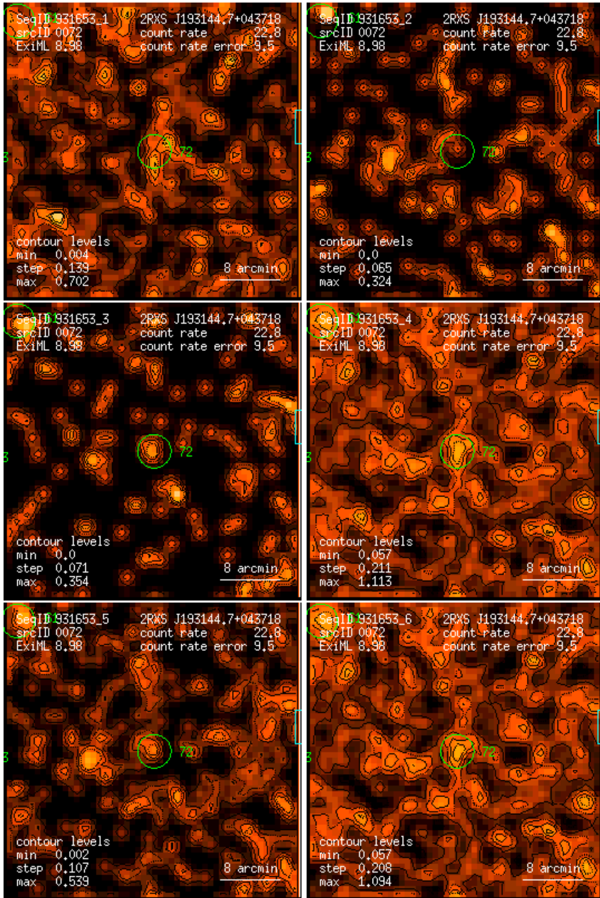
Figure 72: RASS 931653: detection 0072: band rate images, Gaussian filter: (1) PSPC channels 11 – 41, (2) 52 – 90, (3) 91 – 201, (4) 11 – 235, (5) 52 – 201, (6) 11 – 201. Broad band rates in counts/ks. Band rate contour levels in counts/ks/arcmin 2 .
