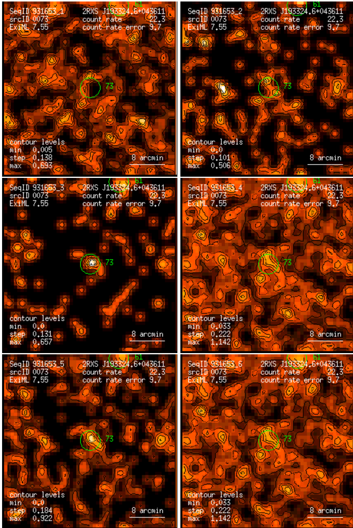
Figure 73: RASS 931653: detection 0073: band rate images, Gaussian filter: (1) PSPC channels 11 – 41, (2) 52 – 90, (3) 91 – 201, (4) 11 – 235, (5) 52 – 201, (6) 11 – 201. Broad band rates in counts/ks. Band rate contour levels in counts/ks/arcmin 2 .
