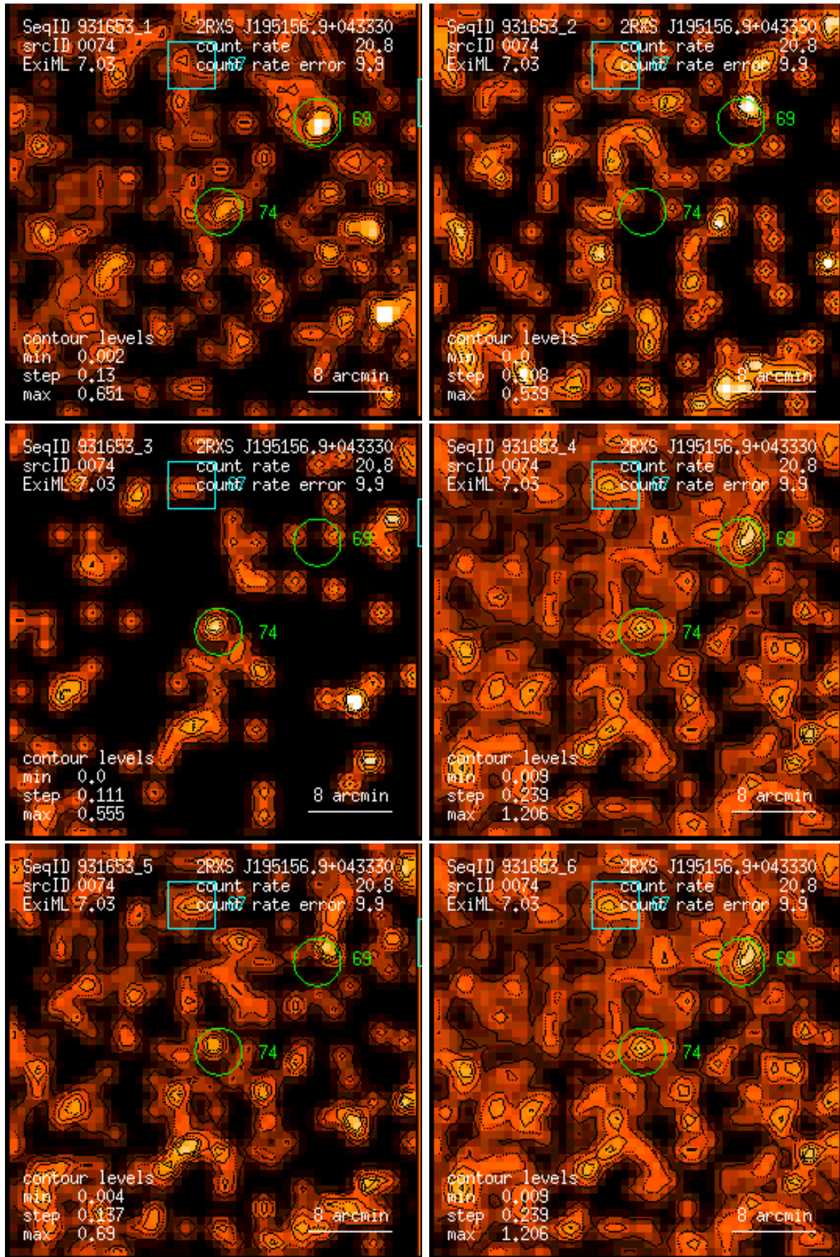
Figure 74: RASS 931653: detection 0074: band rate images, Gaussian filter: (1) PSPC channels 11 – 41, (2) 52 – 90, (3) 91 – 201, (4) 11 – 235, (5) 52 – 201, (6) 11 – 201. Broad band rates in counts/ks. Band rate contour levels in counts/ks/arcmin 2 .
