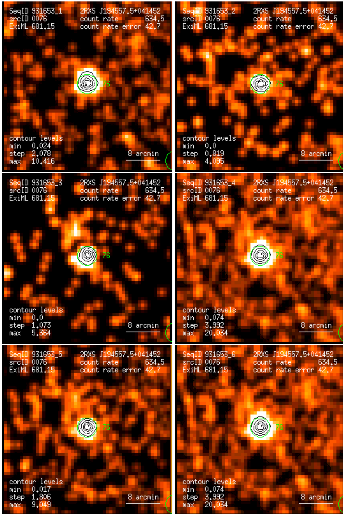
Figure 76: RASS 931653: detection 0076: band rate images, Gaussian filter: (1) PSPC channels 11 – 41, (2) 52 – 90, (3) 91 – 201, (4) 11 – 235, (5) 52 – 201, (6) 11 – 201. Broad band rates in counts/ks. Band rate contour levels in counts/ks/arcmin 2 .
