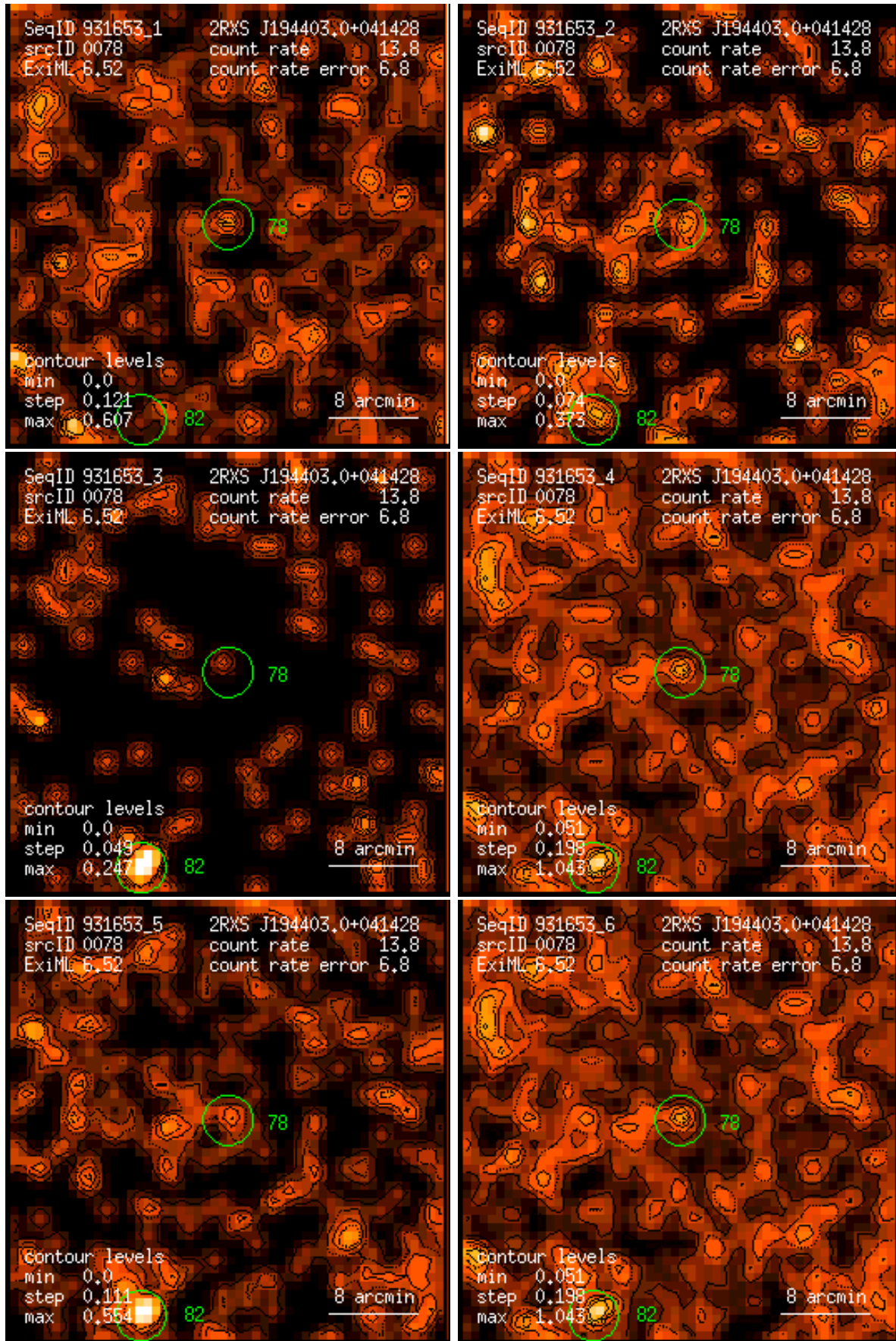
Figure 78: RASS 931653: detection 0078: band rate images, Gaussian filter: (1) PSPC channels 11 – 41, (2) 52 – 90, (3) 91 – 201, (4) 11 – 235, (5) 52 – 201, (6) 11 – 201. Broad band rates in counts/ks. Band rate contour levels in counts/ks/arcmin 2 .
