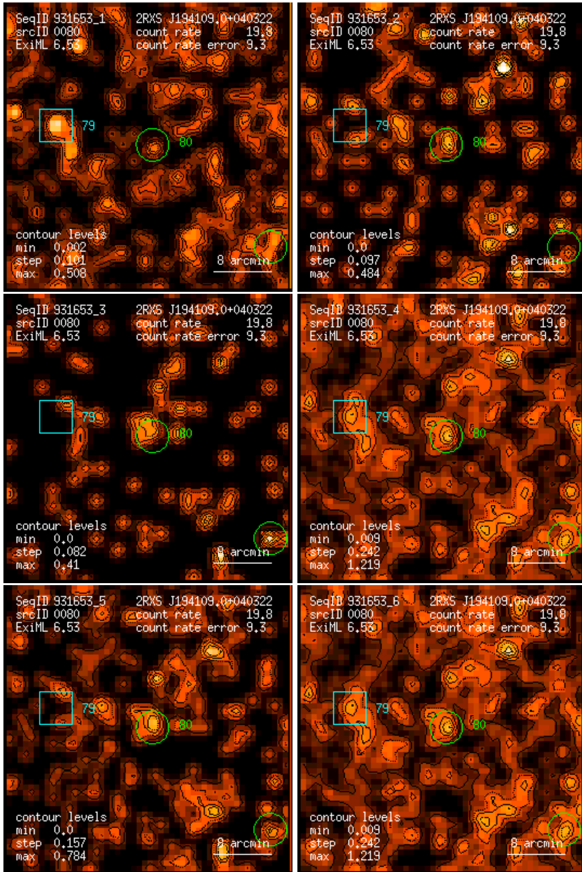
Figure 80: RASS 931653: detection 0080: band rate images, Gaussian filter: (1) PSPC channels 11 – 41, (2) 52 – 90, (3) 91 – 201, (4) 11 – 235, (5) 52 – 201, (6) 11 – 201. Broad band rates in counts/ks. Band rate contour levels in counts/ks/arcmin 2 .
