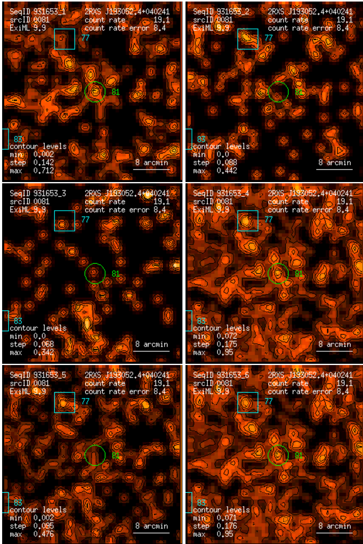
Figure 81: RASS 931653: detection 0081: band rate images, Gaussian filter: (1) PSPC channels 11 – 41, (2) 52 – 90, (3) 91 – 201, (4) 11 – 235, (5) 52 – 201, (6) 11 – 201. Broad band rates in counts/ks. Band rate contour levels in counts/ks/arcmin 2 .
