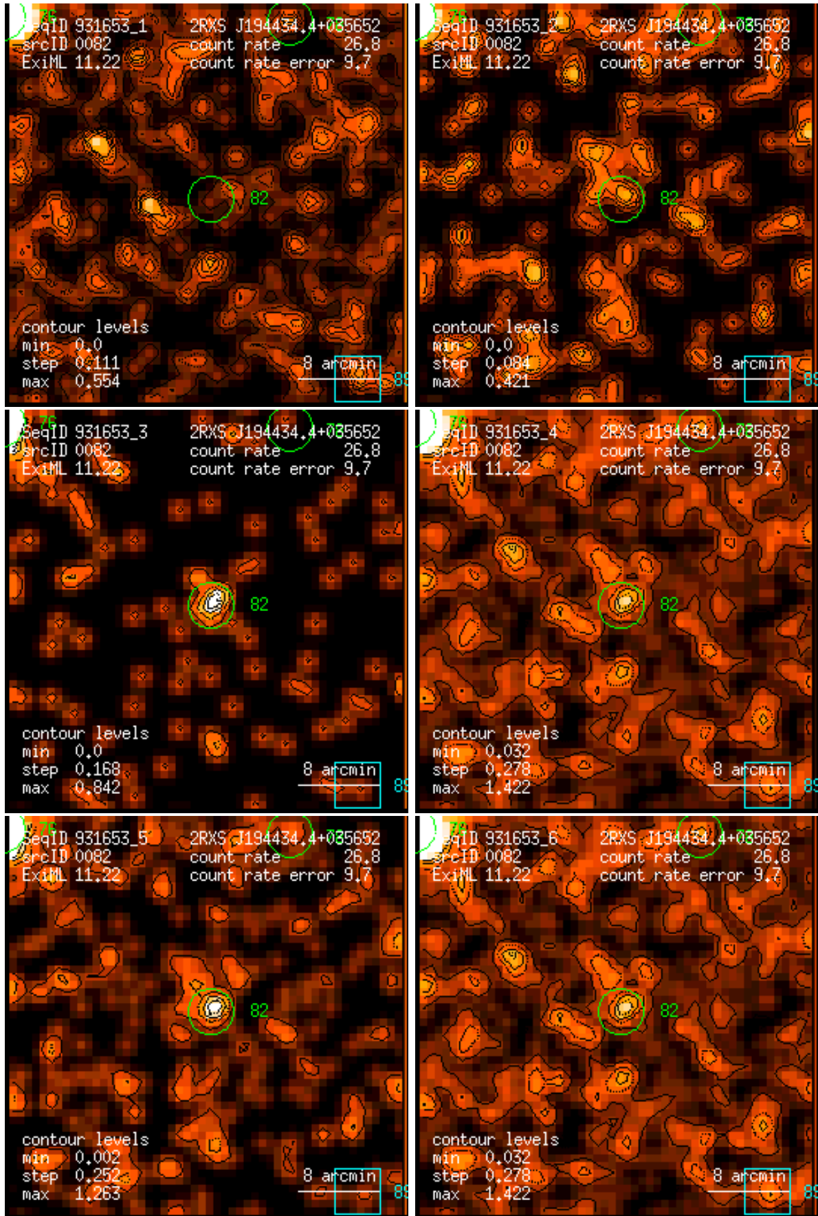
Figure 82: RASS 931653: detection 0082: band rate images, Gaussian filter: (1) PSPC channels 11 – 41, (2) 52 – 90, (3) 91 – 201, (4) 11 – 235, (5) 52 – 201, (6) 11 – 201. Broad band rates in counts/ks. Band rate contour levels in counts/ks/arcmin 2 .
