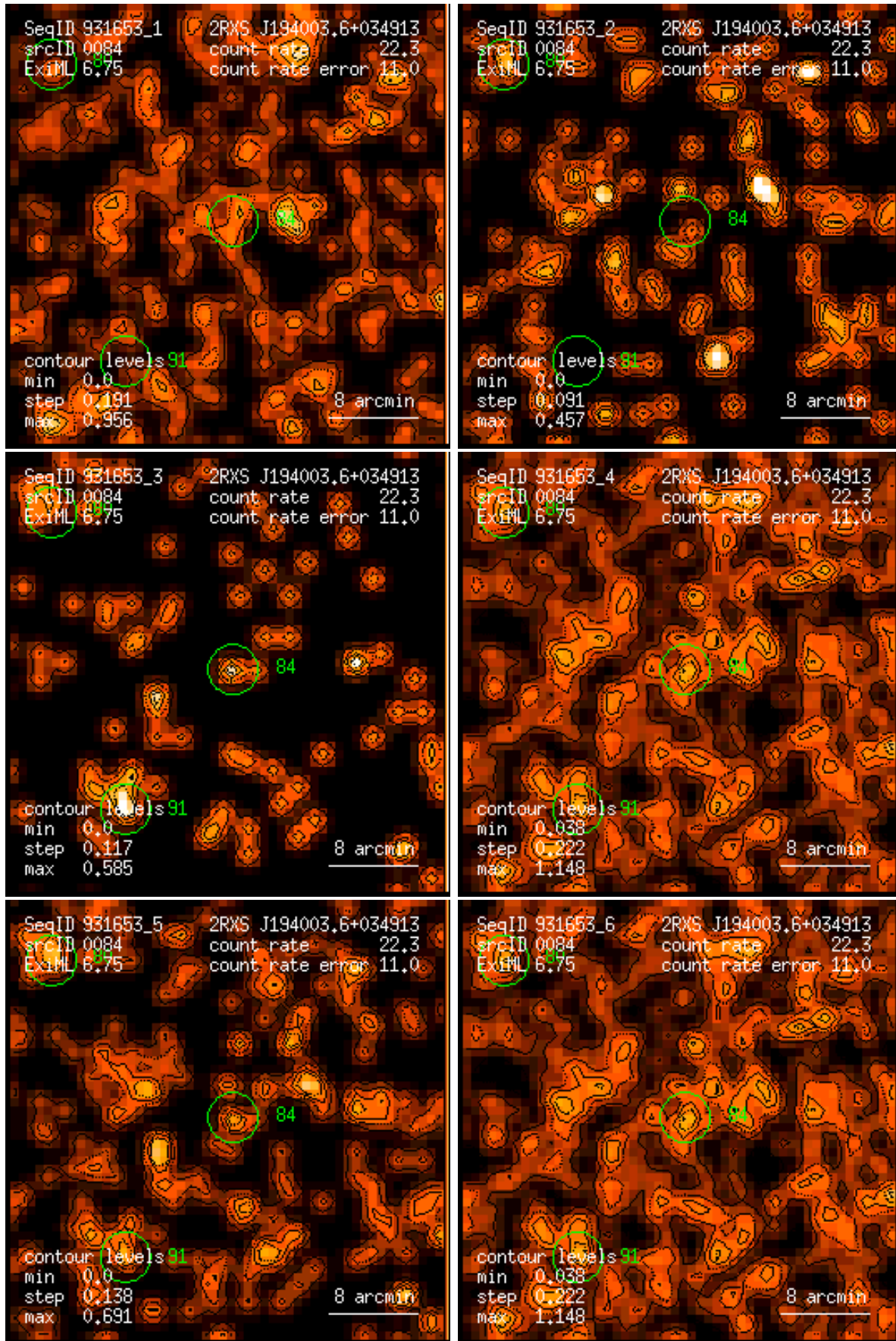
Figure 84: RASS 931653: detection 0084: band rate images, Gaussian filter: (1) PSPC channels 11 – 41, (2) 52 – 90, (3) 91 – 201, (4) 11 – 235, (5) 52 – 201, (6) 11 – 201. Broad band rates in counts/ks. Band rate contour levels in counts/ks/arcmin 2 .
