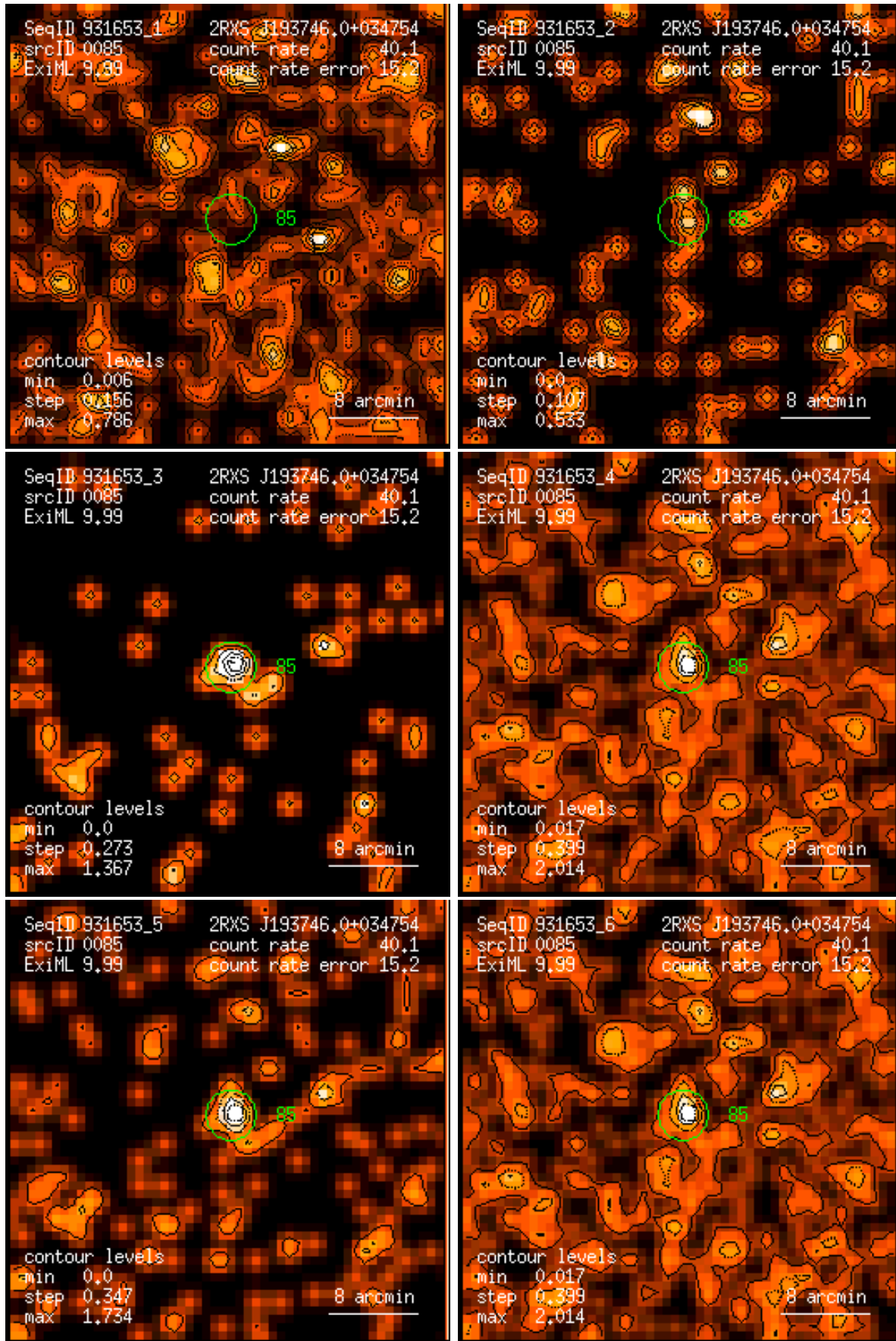
Figure 85: RASS 931653: detection 0085: band rate images, Gaussian filter: (1) PSPC channels 11 – 41, (2) 52 – 90, (3) 91 – 201, (4) 11 – 235, (5) 52 – 201, (6) 11 – 201. Broad band rates in counts/ks. Band rate contour levels in counts/ks/arcmin 2 .
