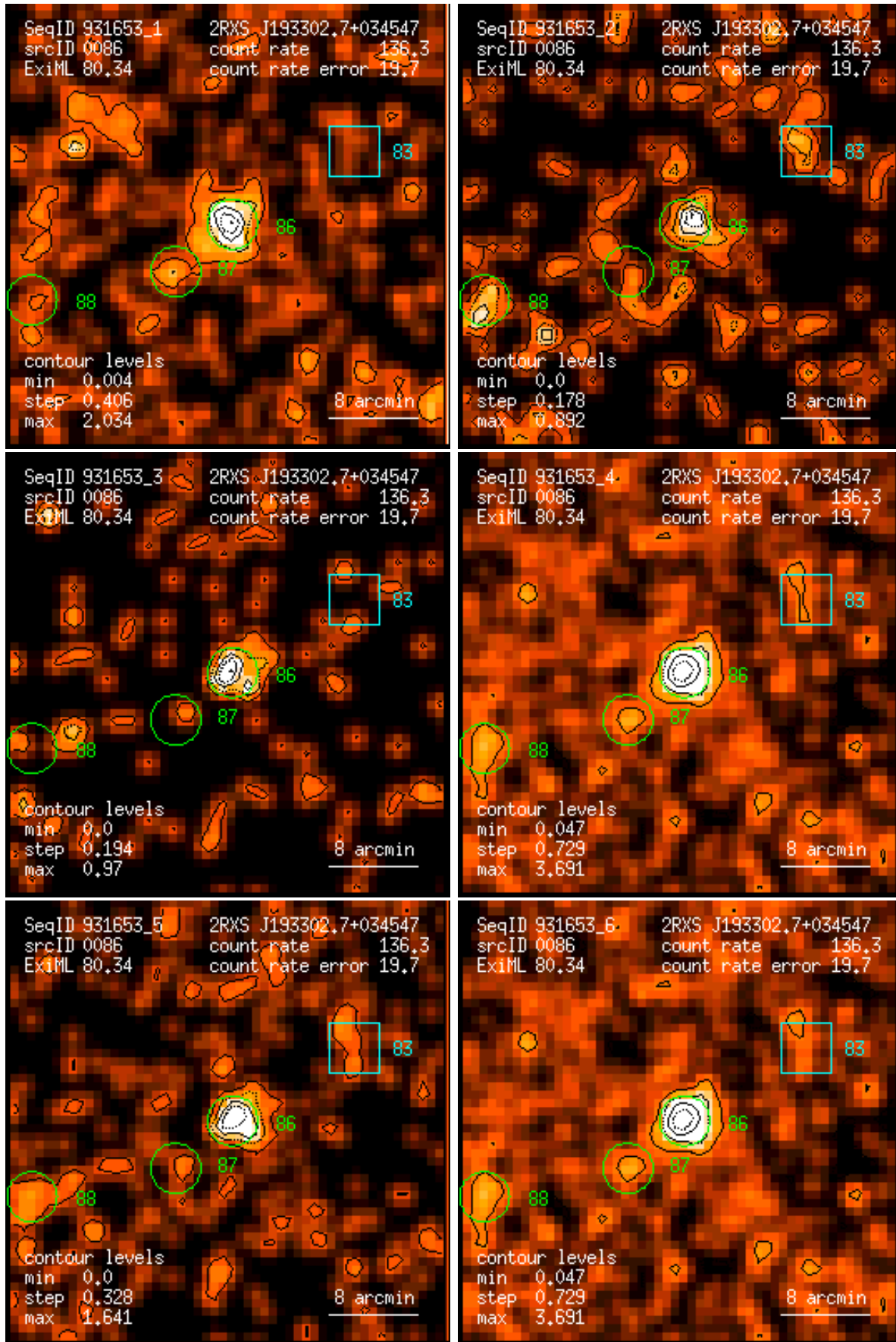
Figure 86: RASS 931653: detection 0086: band rate images, Gaussian filter: (1) PSPC channels 11 – 41, (2) 52 – 90, (3) 91 – 201, (4) 11 – 235, (5) 52 – 201, (6) 11 – 201. Broad band rates in counts/ks. Band rate contour levels in counts/ks/arcmin 2 .
