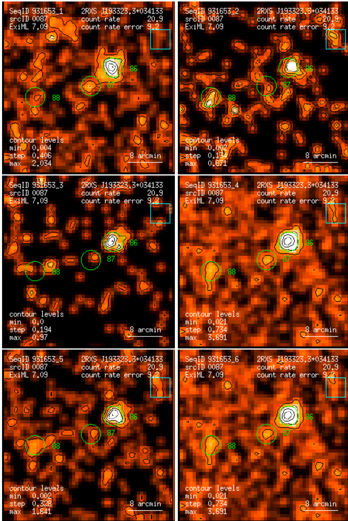
Figure 87: RASS 931653: detection 0087: band rate images, Gaussian filter: (1) PSPC channels 11 – 41, (2) 52 – 90, (3) 91 – 201, (4) 11 – 235, (5) 52 – 201, (6) 11 – 201. Broad band rates in counts/ks. Band rate contour levels in counts/ks/arcmin 2 .
