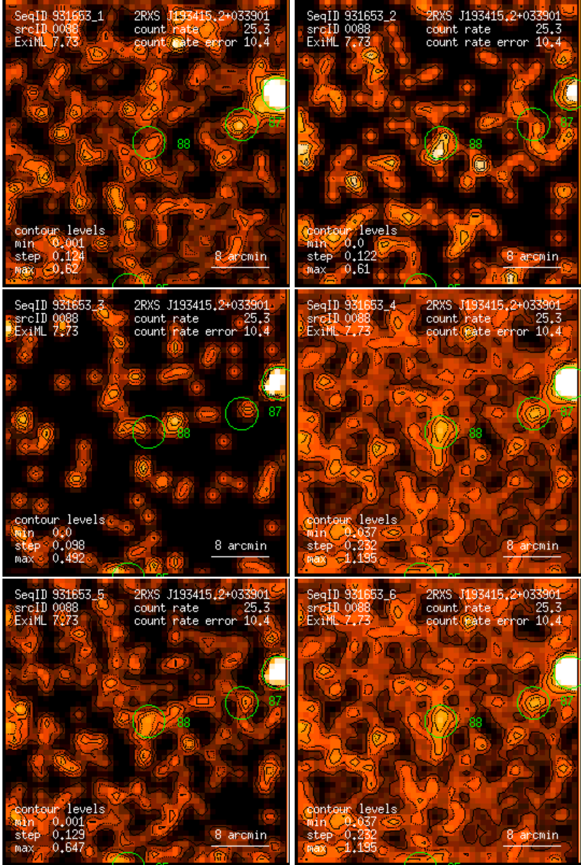
Figure 88: RASS 931653: detection 0088: band rate images, Gaussian filter: (1) PSPC channels 11 – 41, (2) 52 – 90, (3) 91 – 201, (4) 11 – 235, (5) 52 – 201, (6) 11 – 201. Broad band rates in counts/ks. Band rate contour levels in counts/ks/arcmin 2 .
