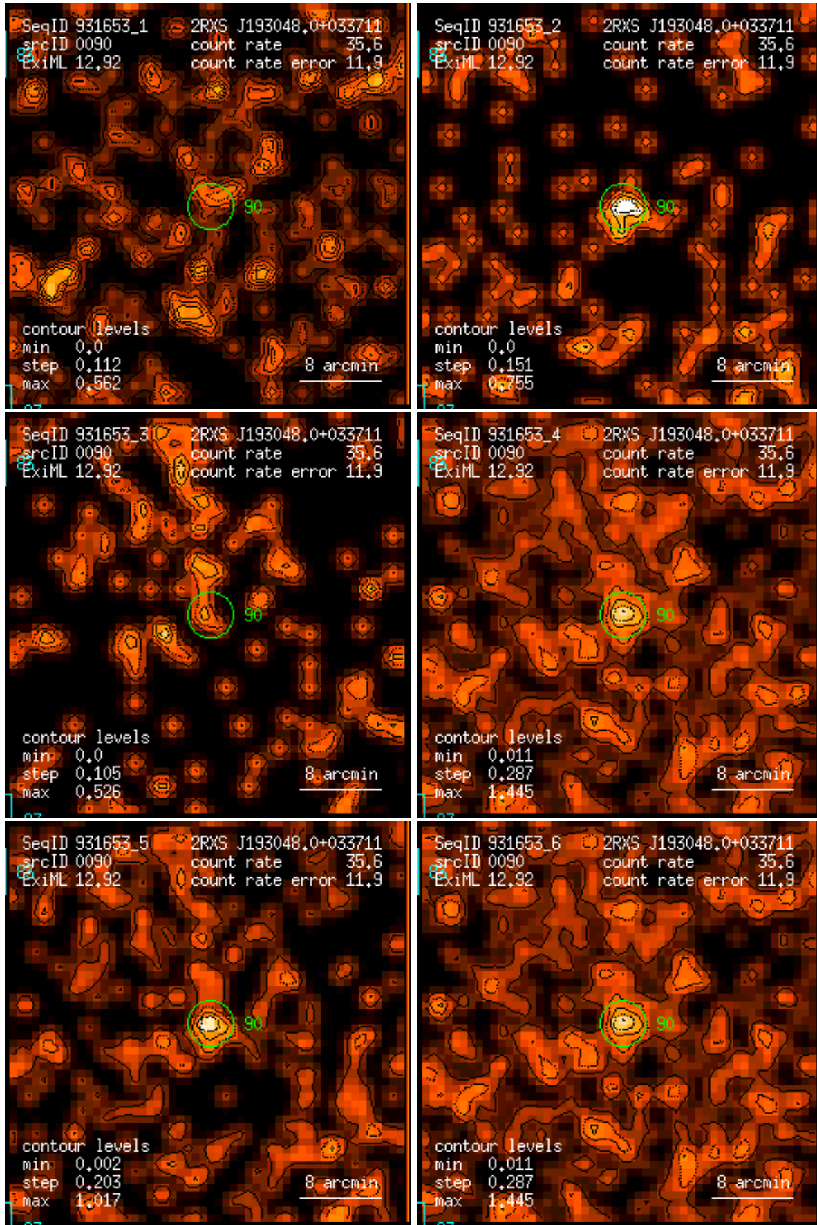
Figure 90: RASS 931653: detection 0090: band rate images, Gaussian filter: (1) PSPC channels 11 – 41, (2) 52 – 90, (3) 91 – 201, (4) 11 – 235, (5) 52 – 201, (6) 11 – 201. Broad band rates in counts/ks. Band rate contour levels in counts/ks/arcmin 2 .
