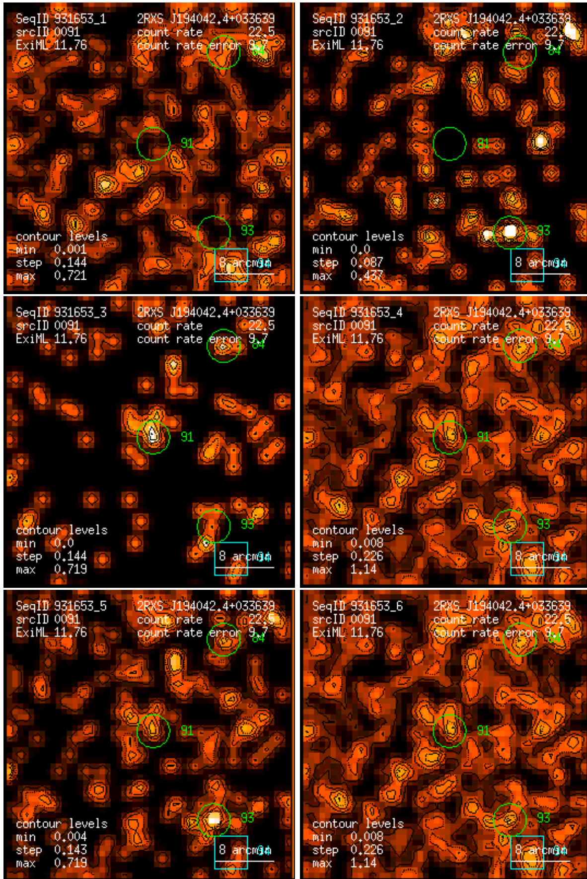
Figure 91: RASS 931653: detection 0091: band rate images, Gaussian filter: (1) PSPC channels 11 – 41, (2) 52 – 90, (3) 91 – 201, (4) 11 – 235, (5) 52 – 201, (6) 11 – 201. Broad band rates in counts/ks. Band rate contour levels in counts/ks/arcmin 2 .
