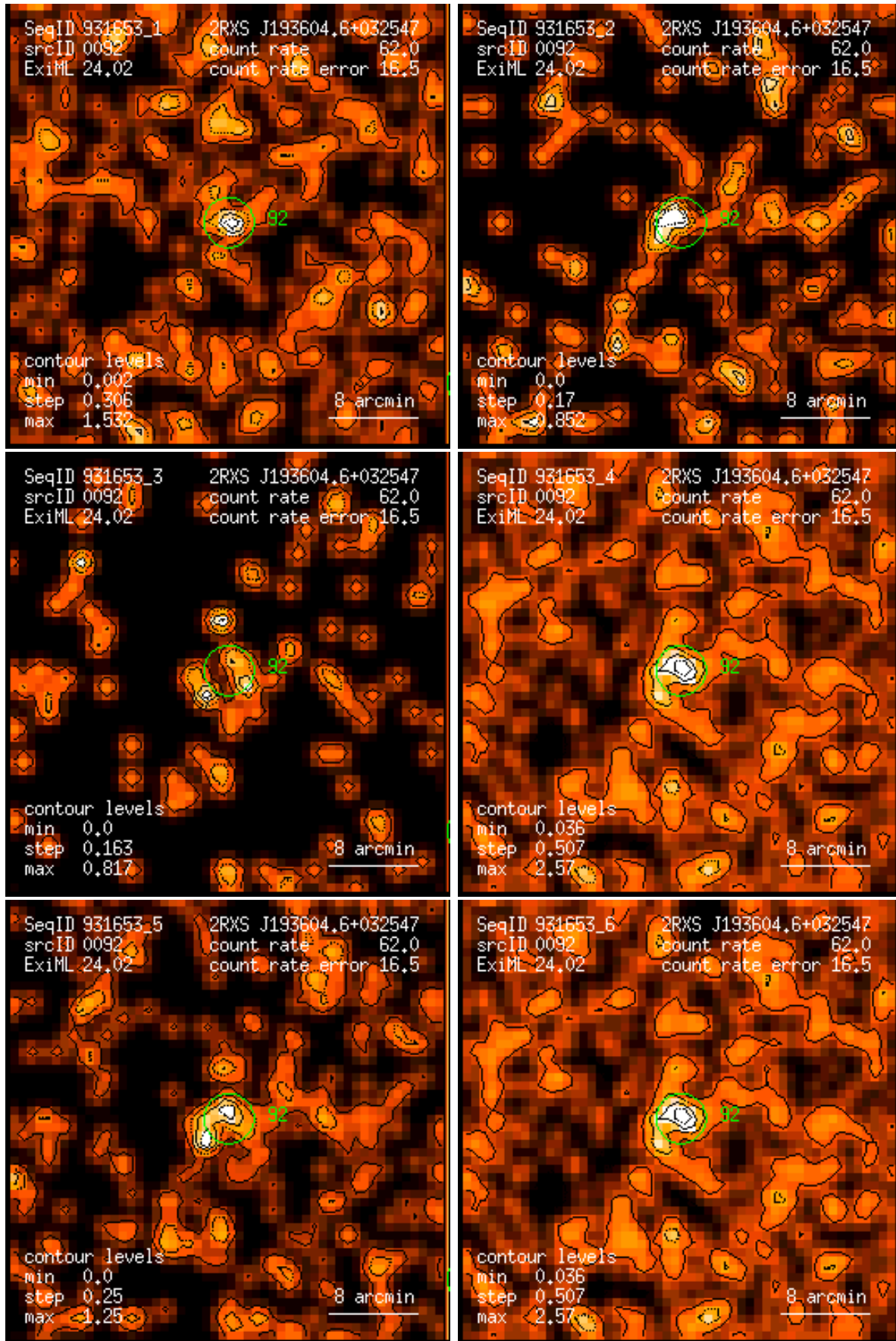
Figure 92: RASS 931653: detection 0092: band rate images, Gaussian filter: (1) PSPC channels 11 – 41, (2) 52 – 90, (3) 91 – 201, (4) 11 – 235, (5) 52 – 201, (6) 11 – 201. Broad band rates in counts/ks. Band rate contour levels in counts/ks/arcmin 2 .
