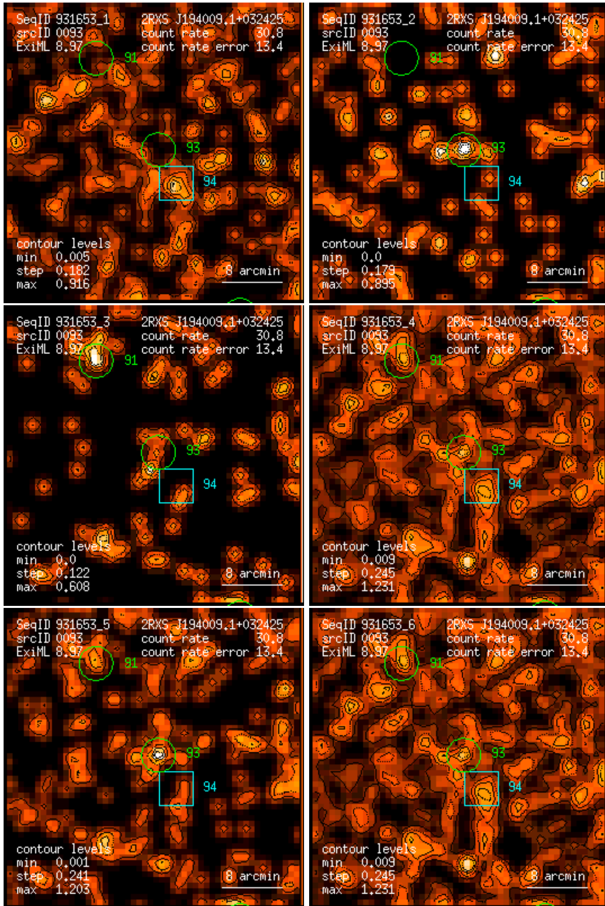
Figure 93: RASS 931653: detection 0093: band rate images, Gaussian filter: (1) PSPC channels 11 – 41, (2) 52 – 90, (3) 91 – 201, (4) 11 – 235, (5) 52 – 201, (6) 11 – 201. Broad band rates in counts/ks. Band rate contour levels in counts/ks/arcmin 2 .
