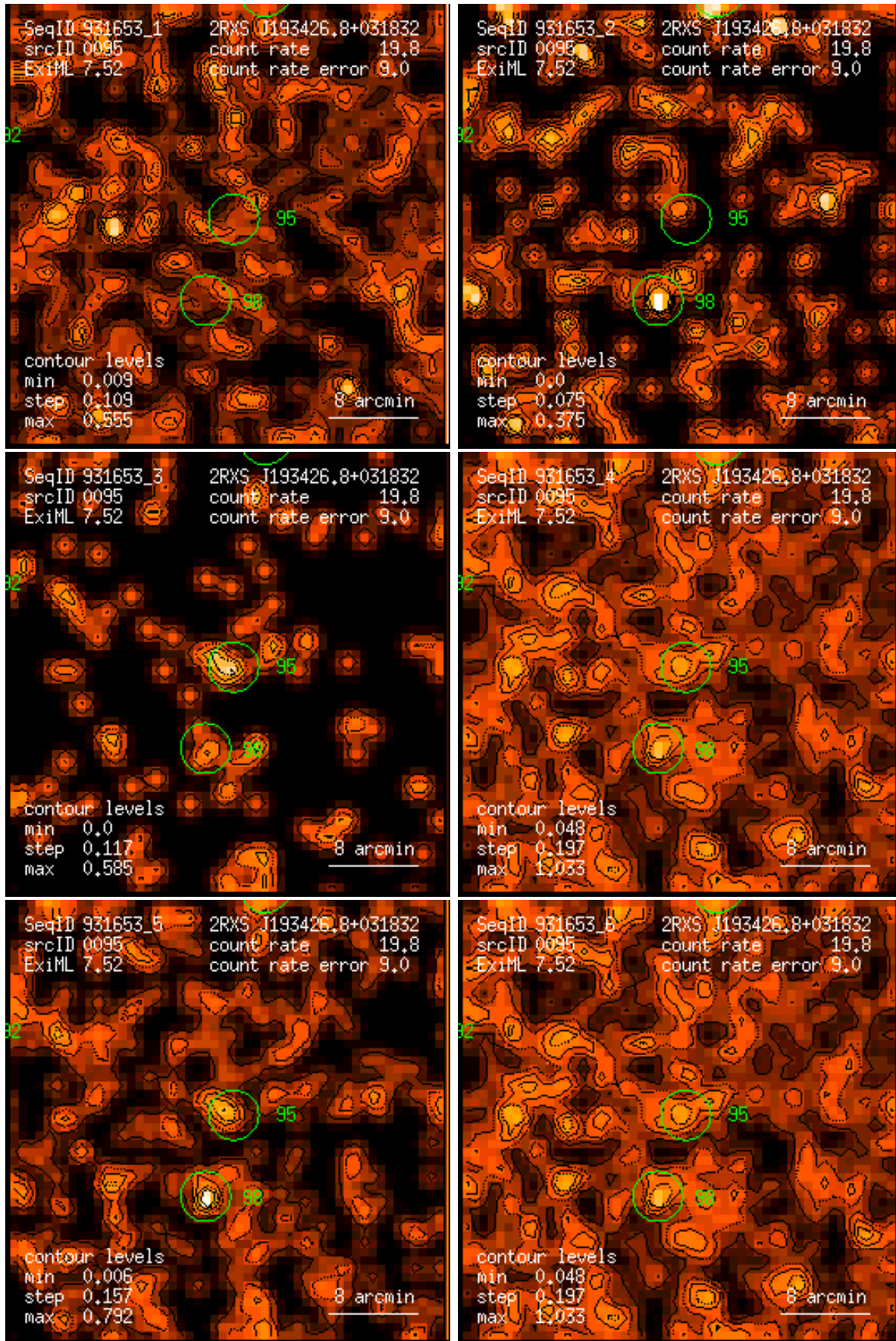
Figure 95: RASS 931653: detection 0095: band rate images, Gaussian filter: (1) PSPC channels 11 – 41, (2) 52 – 90, (3) 91 – 201, (4) 11 – 235, (5) 52 – 201, (6) 11 – 201. Broad band rates in counts/ks. Band rate contour levels in counts/ks/arcmin 2 .
