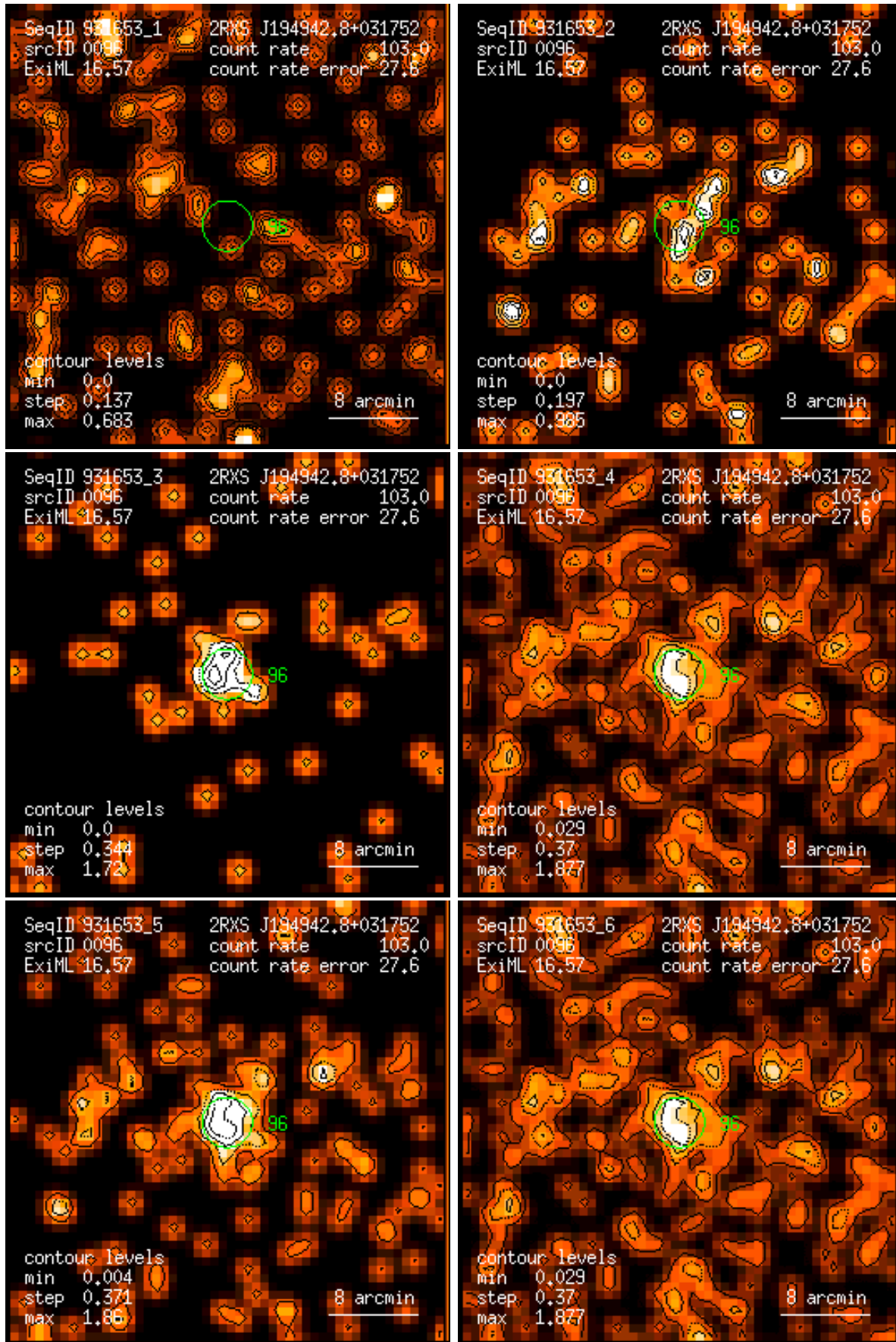
Figure 96: RASS 931653: detection 0096: band rate images, Gaussian filter: (1) PSPC channels 11 – 41, (2) 52 – 90, (3) 91 – 201, (4) 11 – 235, (5) 52 – 201, (6) 11 – 201. Broad band rates in counts/ks. Band rate contour levels in counts/ks/arcmin 2 .
