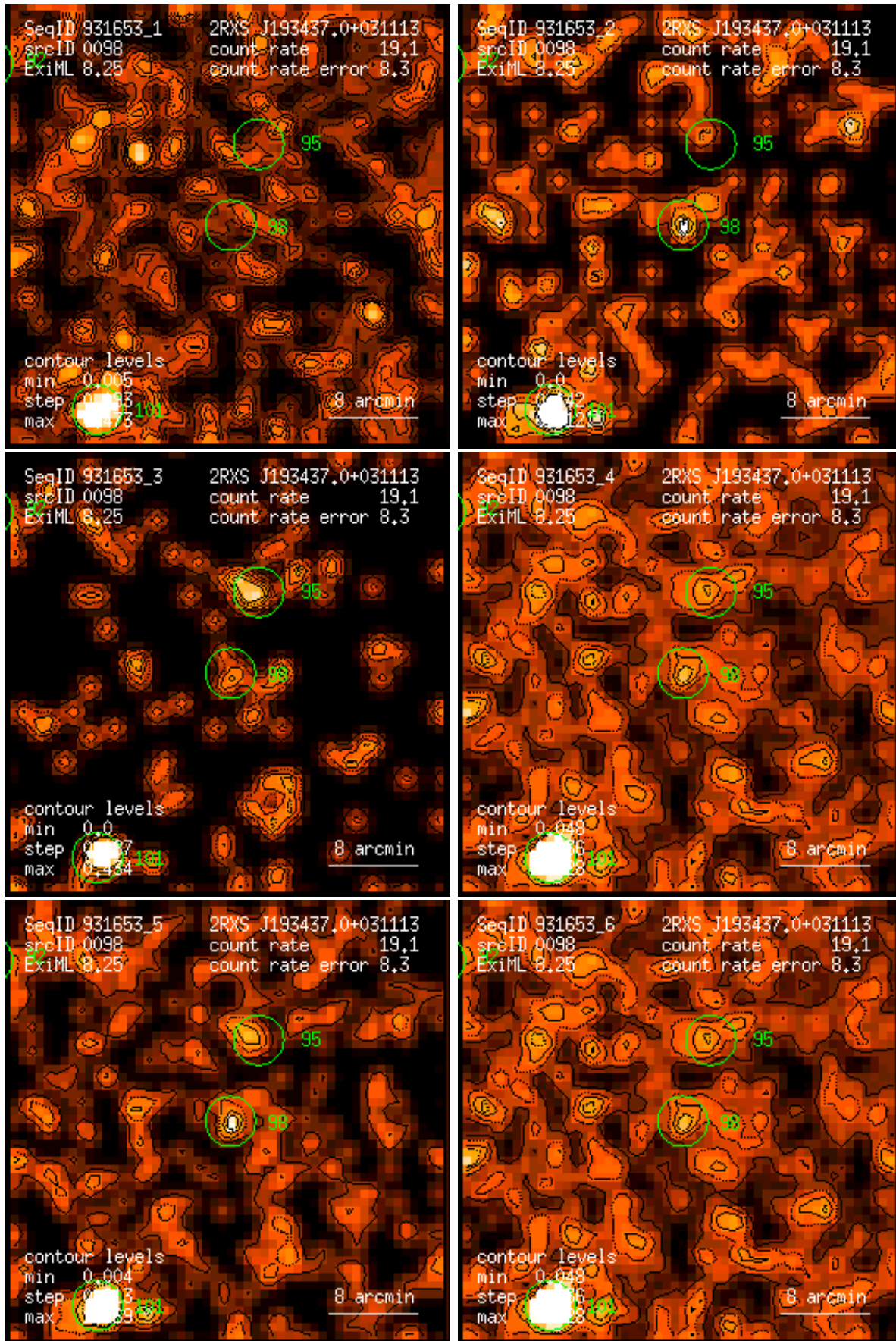
Figure 98: RASS 931653: detection 0098: band rate images, Gaussian filter: (1) PSPC channels 11 – 41, (2) 52 – 90, (3) 91 – 201, (4) 11 – 235, (5) 52 – 201, (6) 11 – 201. Broad band rates in counts/ks. Band rate contour levels in counts/ks/arcmin 2 .
