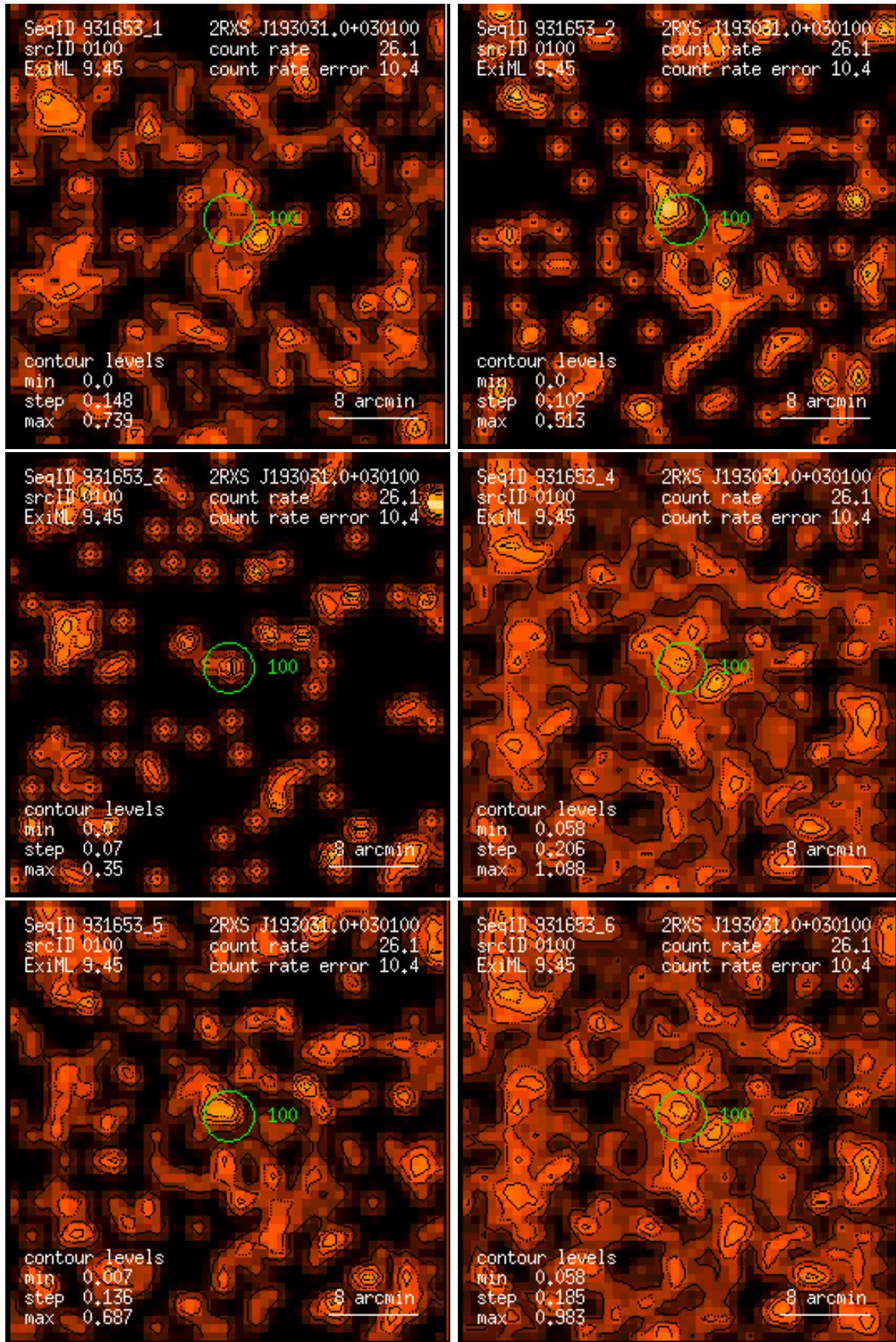
Figure 100: RASS 931653: detection 0100: band rate images, Gaussian filter: (1) PSPC channels 11 – 41, (2) 52 – 90, (3) 91 – 201, (4) 11 – 235, (5) 52 – 201, (6) 11 – 201. Broad band rates in counts/ks. Band rate contour levels in counts/ks/arcmin 2 .
