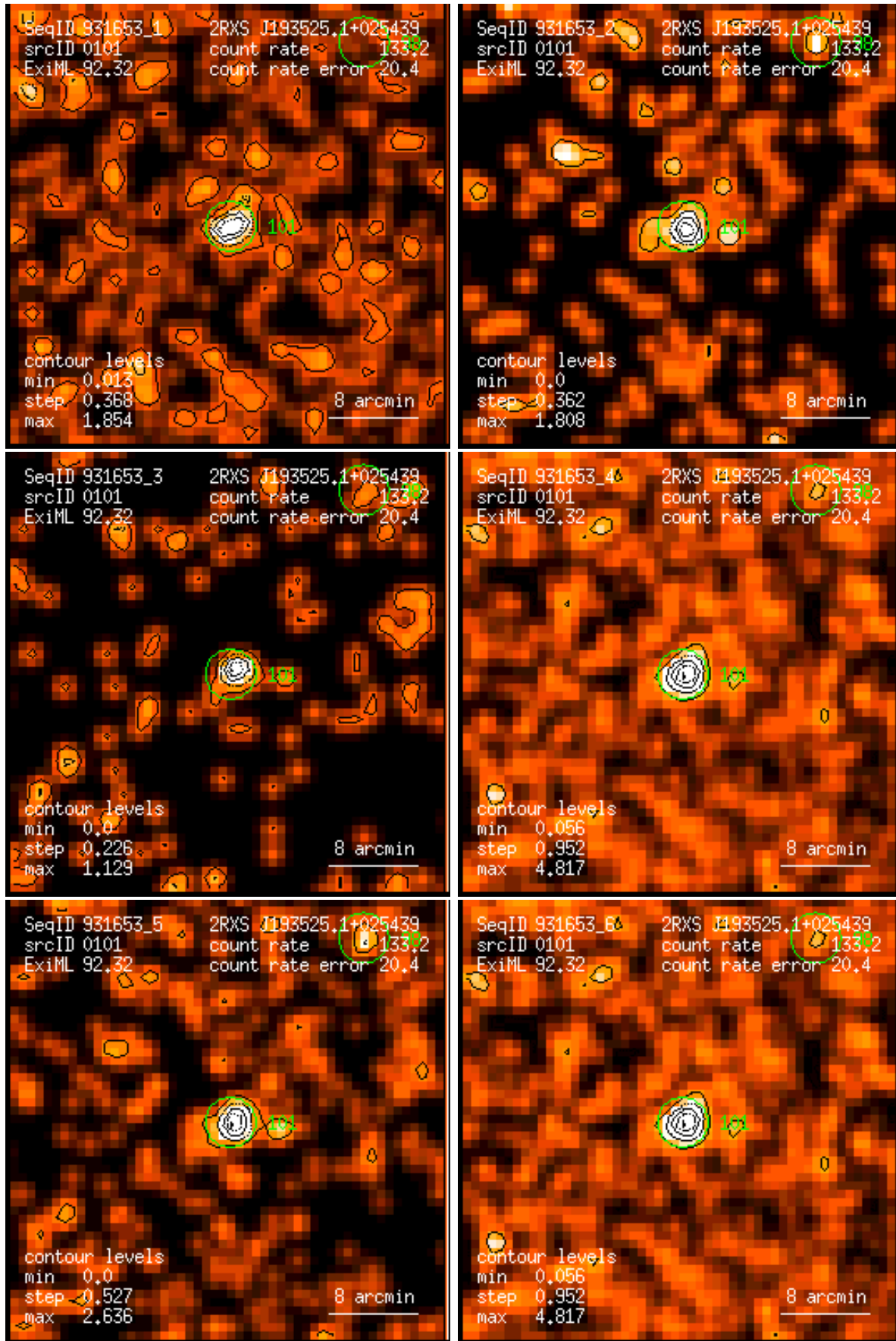
Figure 101: RASS 931653: detection 0101: band rate images, Gaussian filter: (1) PSPC channels 11 – 41, (2) 52 – 90, (3) 91 – 201, (4) 11 – 235, (5) 52 – 201, (6) 11 – 201. Broad band rates in counts/ks. Band rate contour levels in counts/ks/arcmin 2 .
