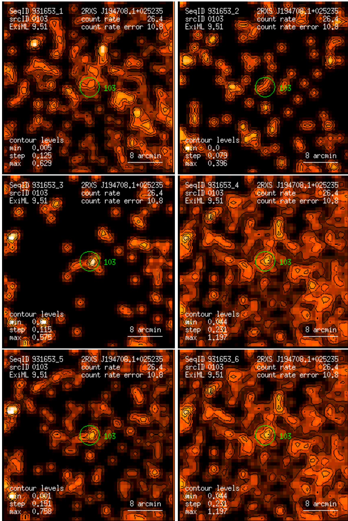
Figure 103: RASS 931653: detection 0103: band rate images, Gaussian filter: (1) PSPC channels 11 – 41, (2) 52 – 90, (3) 91 – 201, (4) 11 – 235, (5) 52 – 201, (6) 11 – 201. Broad band rates in counts/ks. Band rate contour levels in counts/ks/arcmin 2 .
