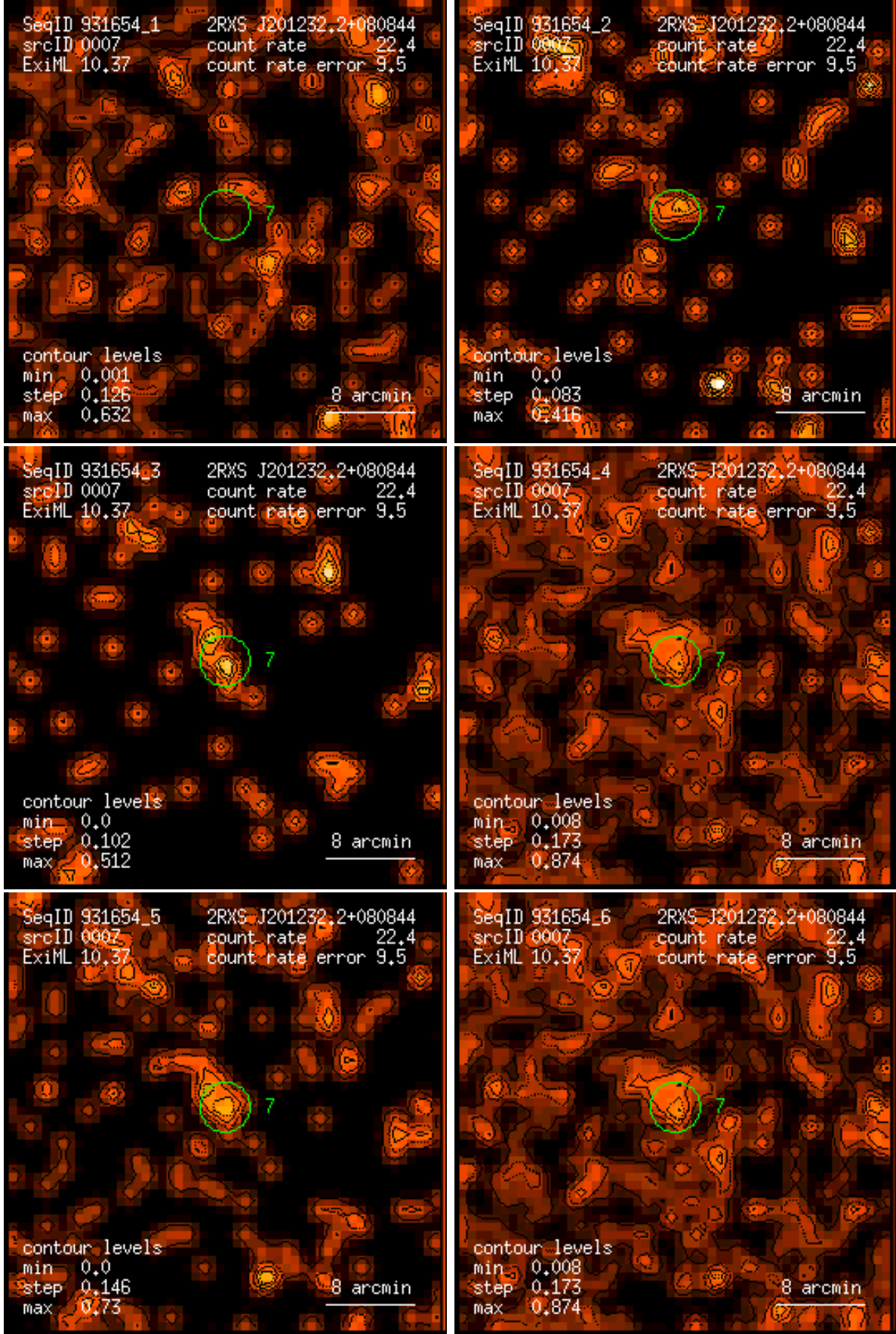
Figure 7: RASS 931654: detection 0007: band rate images, Gaussian filter: (1) PSPC channels 11 – 41, (2) 52 – 90, (3) 91 – 201, (4) 11 – 235, (5) 52 – 201, (6) 11 – 201. Broad band rates in counts/ks. Band rate contour levels in counts/ks/arcmin 2 .
