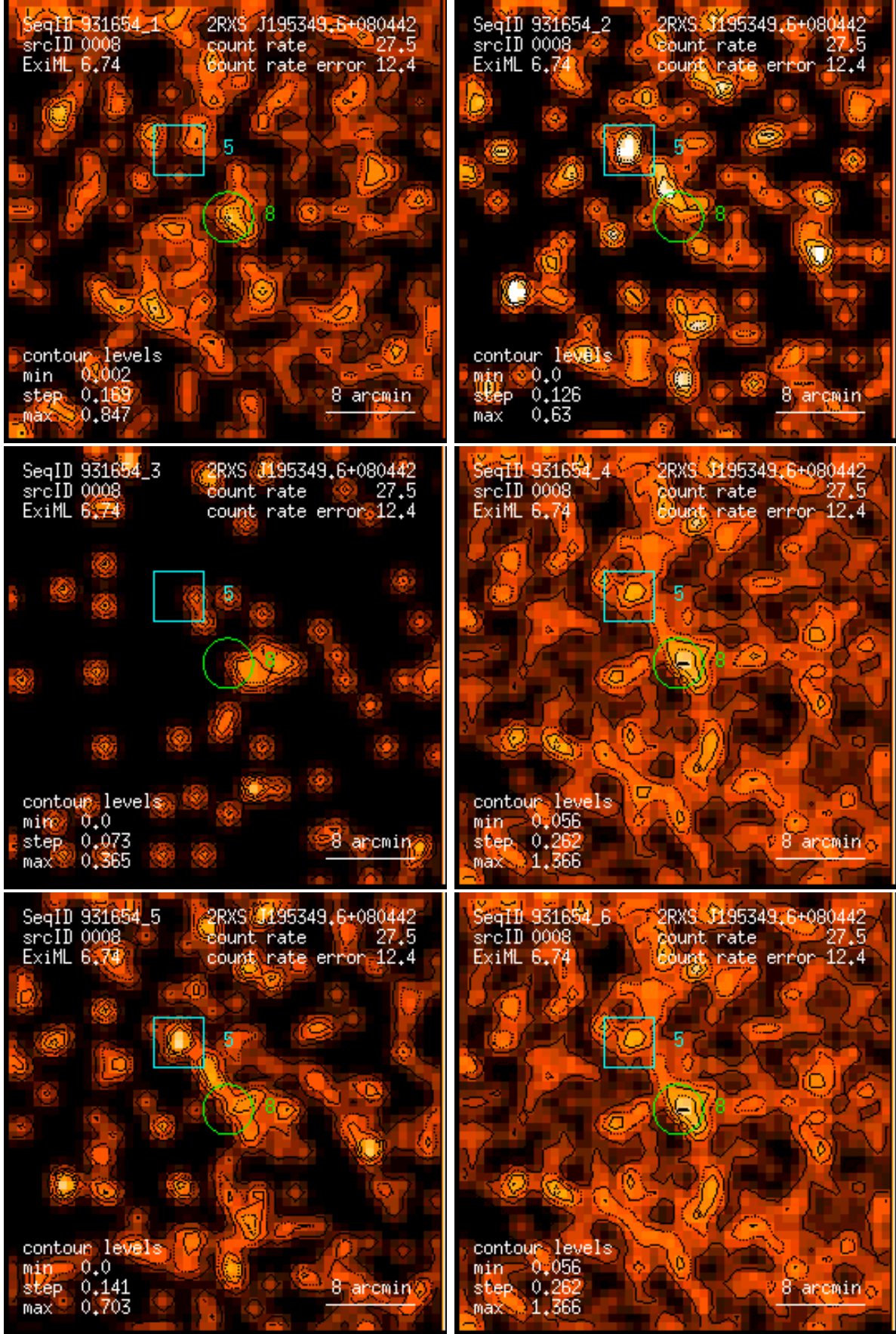
Figure 8: RASS 931654: detection 0008: band rate images, Gaussian filter: (1) PSPC channels 11 – 41, (2) 52 – 90, (3) 91 – 201, (4) 11 – 235, (5) 52 – 201, (6) 11 – 201. Broad band rates in counts/ks. Band rate contour levels in counts/ks/arcmin 2 .
