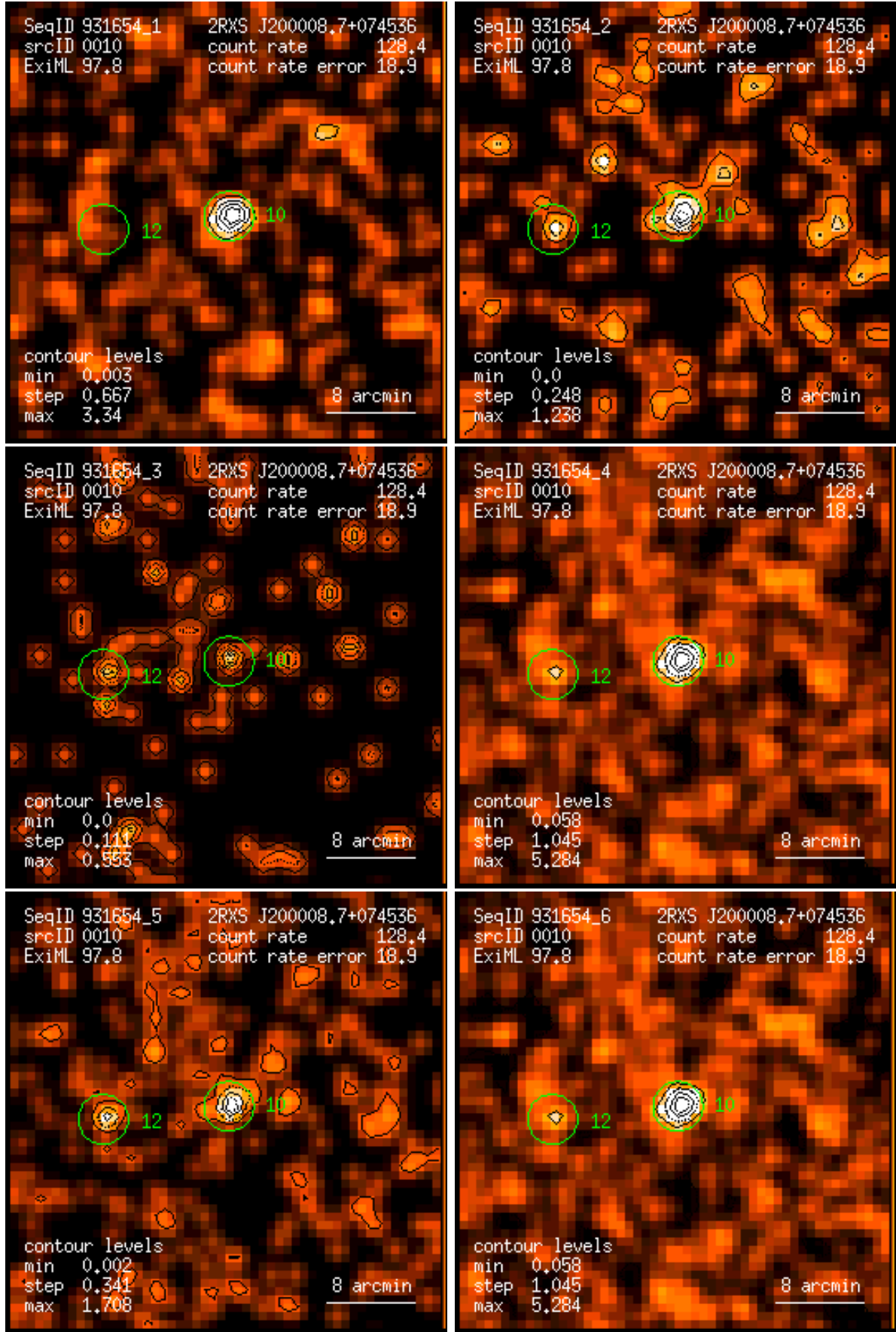
Figure 10: RASS 931654: detection 0010: band rate images, Gaussian filter: (1) PSPC channels 11 – 41, (2) 52 – 90, (3) 91 – 201, (4) 11 – 235, (5) 52 – 201, (6) 11 – 201. Broad band rates in counts/ks. Band rate contour levels in counts/ks/arcmin 2 .
