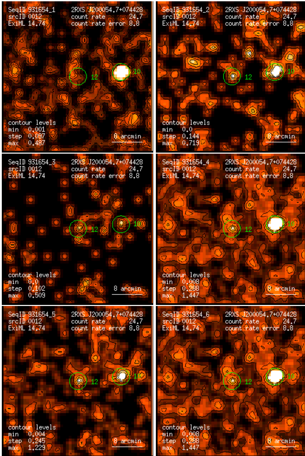
Figure 12: RASS 931654: detection 0012: band rate images, Gaussian filter: (1) PSPC channels 11 – 41, (2) 52 – 90, (3) 91 – 201, (4) 11 – 235, (5) 52 – 201, (6) 11 – 201. Broad band rates in counts/ks. Band rate contour levels in counts/ks/arcmin 2 .
