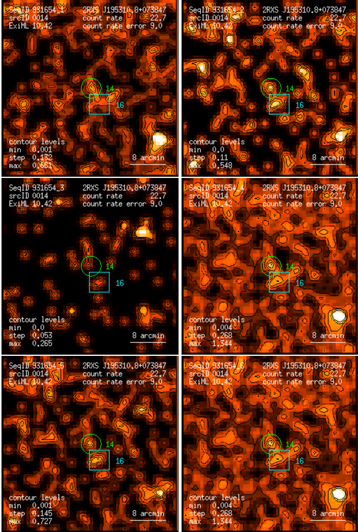
Figure 14: RASS 931654: detection 0014: band rate images, Gaussian filter: (1) PSPC channels 11 – 41, (2) 52 – 90, (3) 91 – 201, (4) 11 – 235, (5) 52 – 201, (6) 11 – 201. Broad band rates in counts/ks. Band rate contour levels in counts/ks/arcmin 2 .
