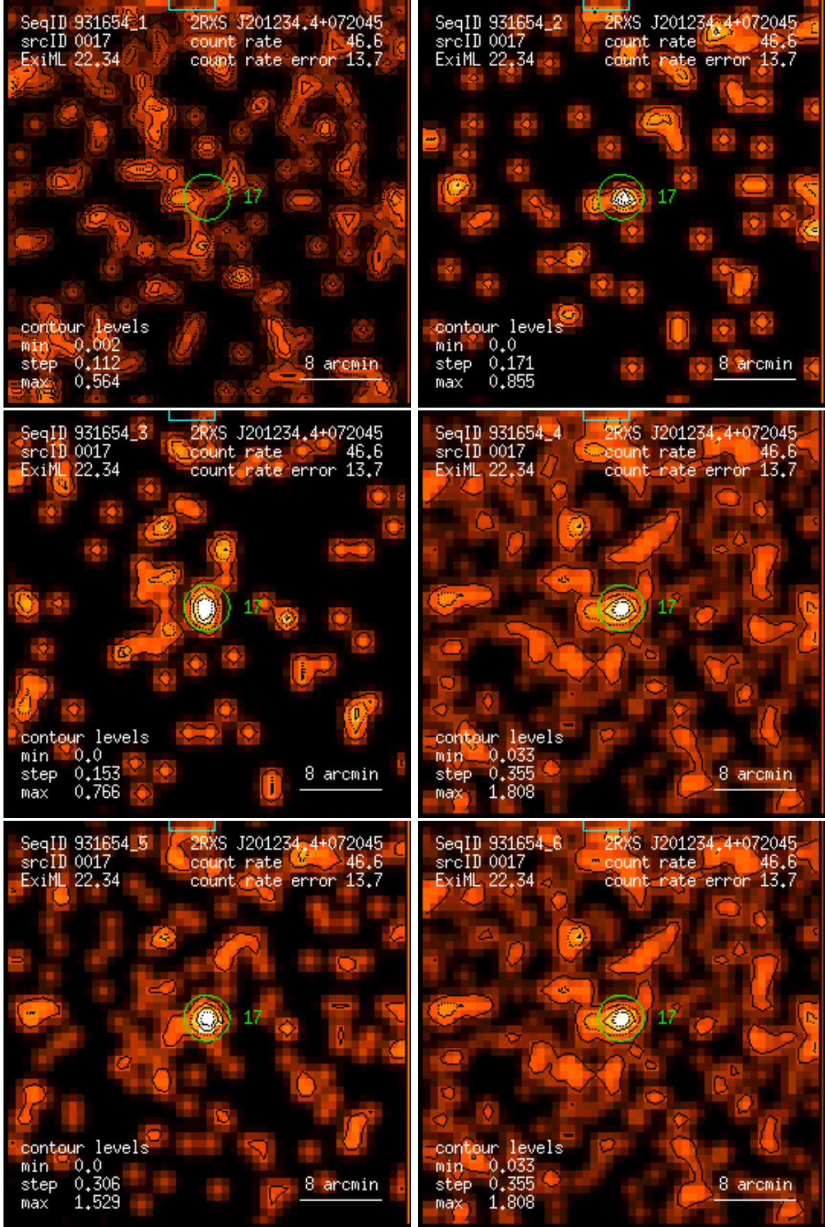
Figure 17: RASS 931654: detection 0017: band rate images, Gaussian filter: (1) PSPC channels 11 – 41, (2) 52 – 90, (3) 91 – 201, (4) 11 – 235, (5) 52 – 201, (6) 11 – 201. Broad band rates in counts/ks. Band rate contour levels in counts/ks/arcmin 2 .
