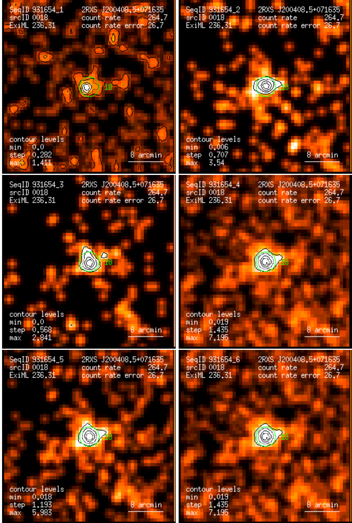
Figure 18: RASS 931654: detection 0018: band rate images, Gaussian filter: (1) PSPC channels 11 – 41, (2) 52 – 90, (3) 91 – 201, (4) 11 – 235, (5) 52 – 201, (6) 11 – 201. Broad band rates in counts/ks. Band rate contour levels in counts/ks/arcmin 2 .
