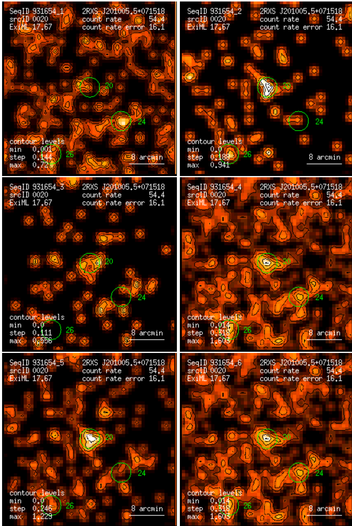
Figure 20: RASS 931654: detection 0020: band rate images, Gaussian filter: (1) PSPC channels 11 – 41, (2) 52 – 90, (3) 91 – 201, (4) 11 – 235, (5) 52 – 201, (6) 11 – 201. Broad band rates in counts/ks. Band rate contour levels in counts/ks/arcmin 2 .
