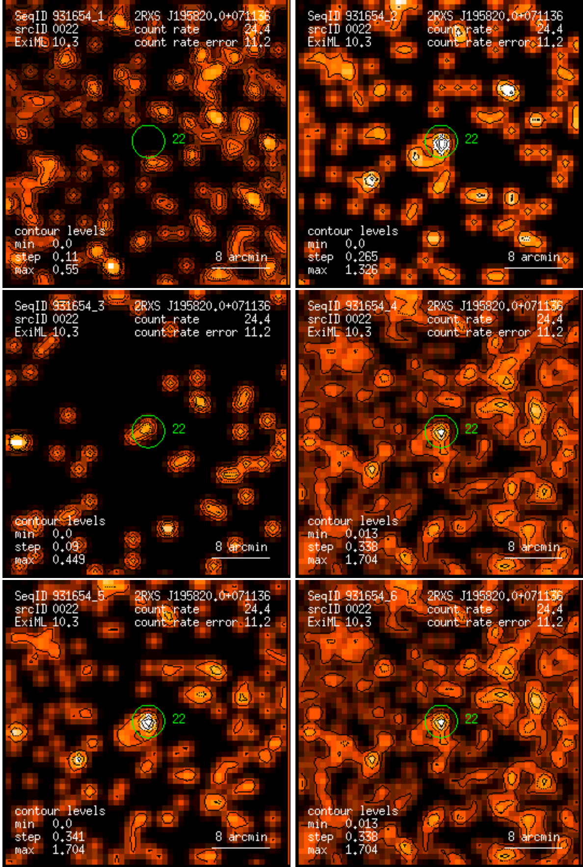
Figure 22: RASS 931654: detection 0022: band rate images, Gaussian filter: (1) PSPC channels 11 – 41, (2) 52 – 90, (3) 91 – 201, (4) 11 – 235, (5) 52 – 201, (6) 11 – 201. Broad band rates in counts/ks. Band rate contour levels in counts/ks/arcmin 2 .
