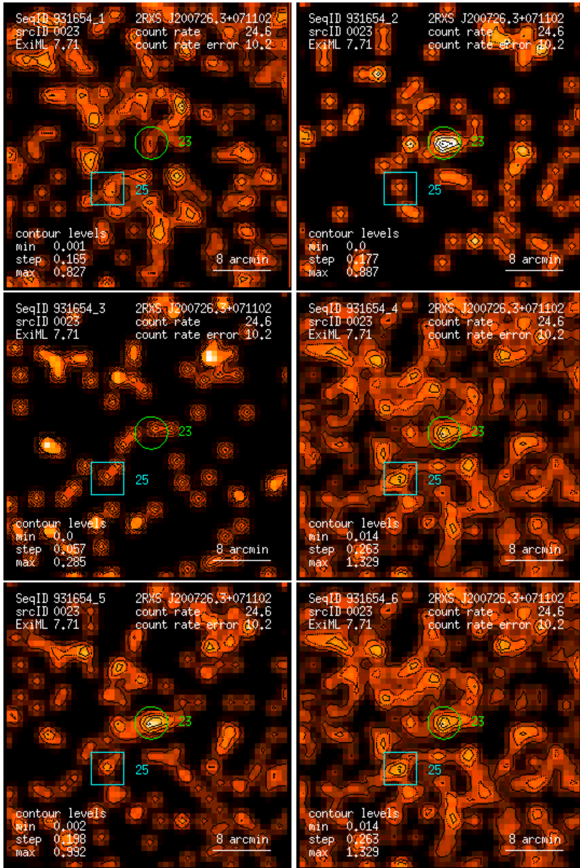
Figure 23: RASS 931654: detection 0023: band rate images, Gaussian filter: (1) PSPC channels 11 – 41, (2) 52 – 90, (3) 91 – 201, (4) 11 – 235, (5) 52 – 201, (6) 11 – 201. Broad band rates in counts/ks. Band rate contour levels in counts/ks/arcmin 2 .
