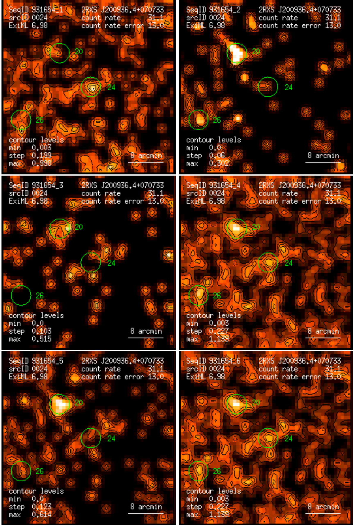
Figure 24: RASS 931654: detection 0024: band rate images, Gaussian filter: (1) PSPC channels 11 – 41, (2) 52 – 90, (3) 91 – 201, (4) 11 – 235, (5) 52 – 201, (6) 11 – 201. Broad band rates in counts/ks. Band rate contour levels in counts/ks/arcmin 2 .
