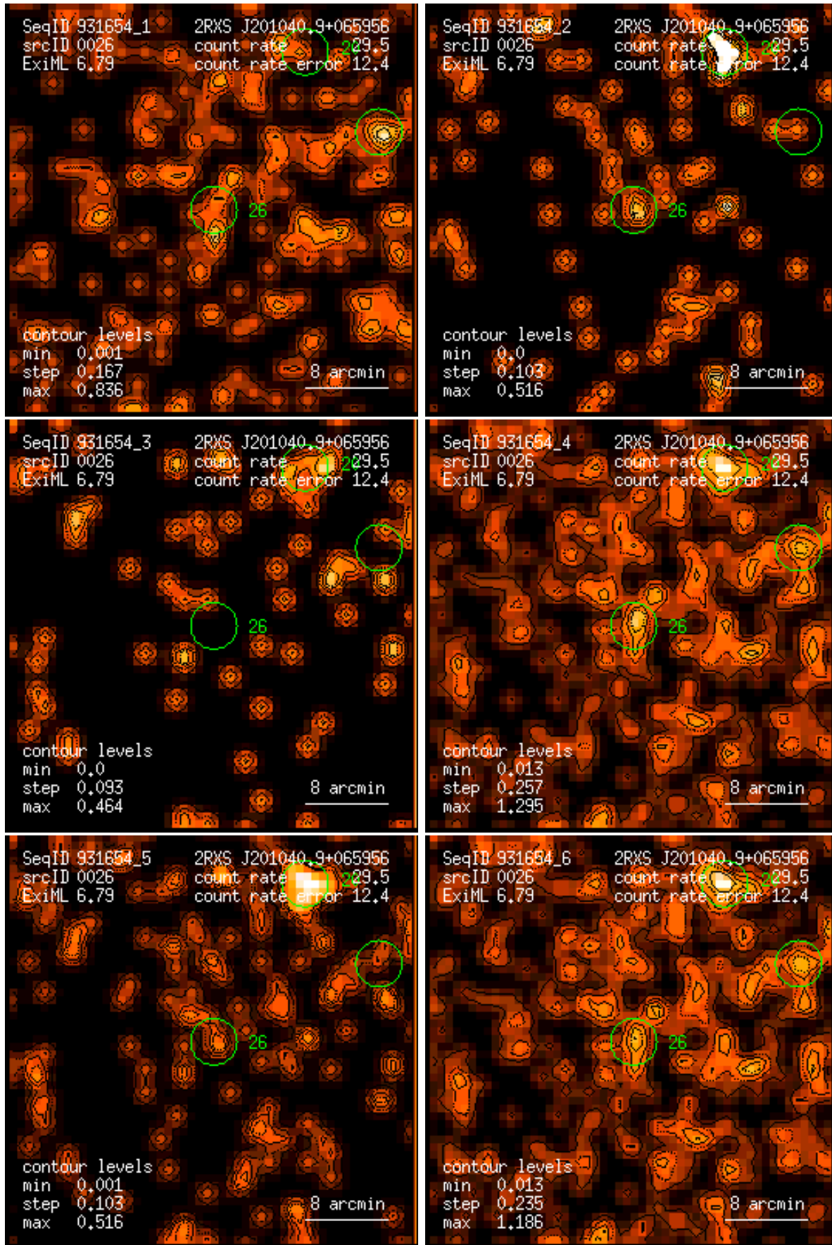
Figure 26: RASS 931654: detection 0026: band rate images, Gaussian filter: (1) PSPC channels 11 – 41, (2) 52 – 90, (3) 91 – 201, (4) 11 – 235, (5) 52 – 201, (6) 11 – 201. Broad band rates in counts/ks. Band rate contour levels in counts/ks/arcmin 2 .
