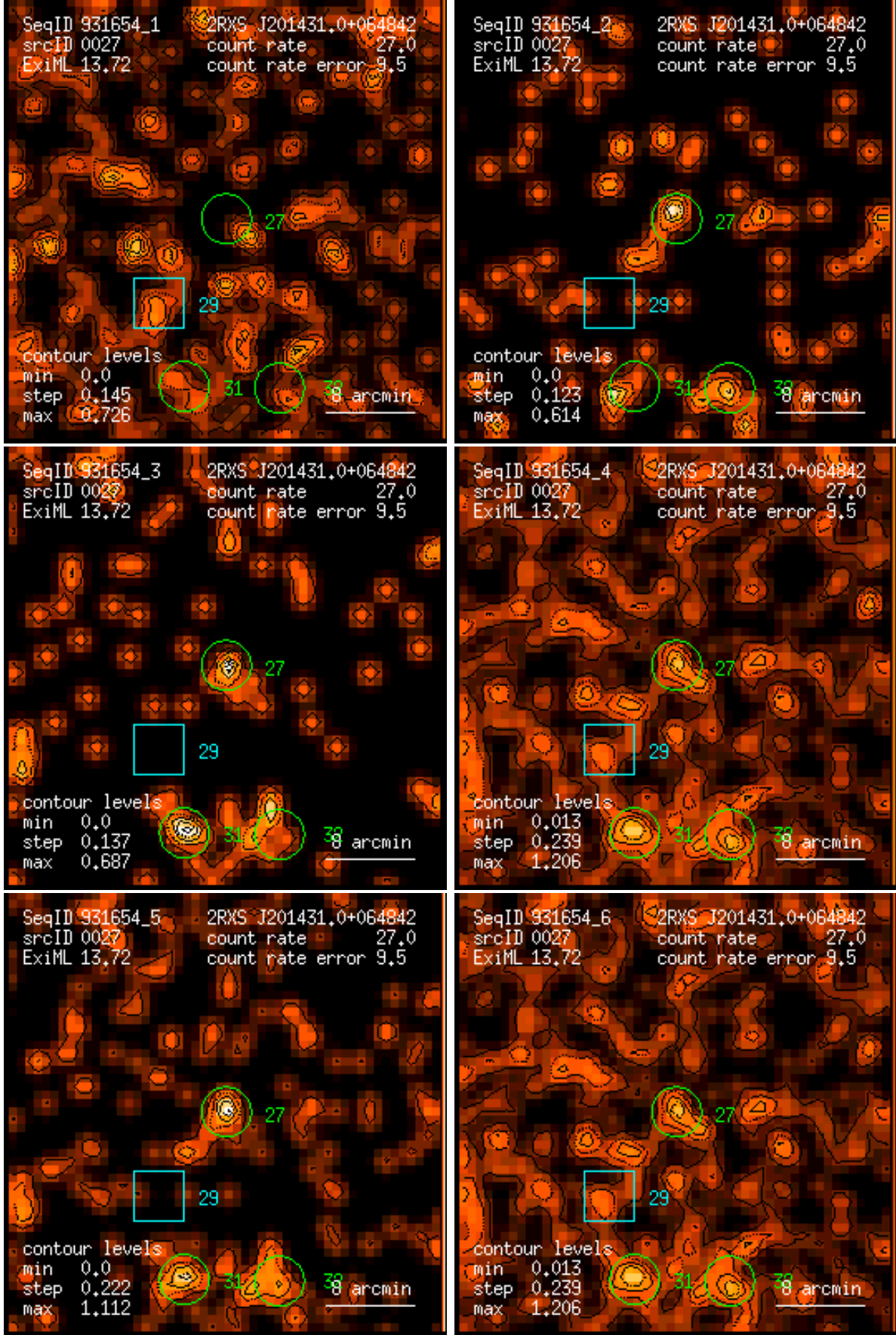
Figure 27: RASS 931654: detection 0027: band rate images, Gaussian filter: (1) PSPC channels 11 – 41, (2) 52 – 90, (3) 91 – 201, (4) 11 – 235, (5) 52 – 201, (6) 11 – 201. Broad band rates in counts/ks. Band rate contour levels in counts/ks/arcmin 2 .
