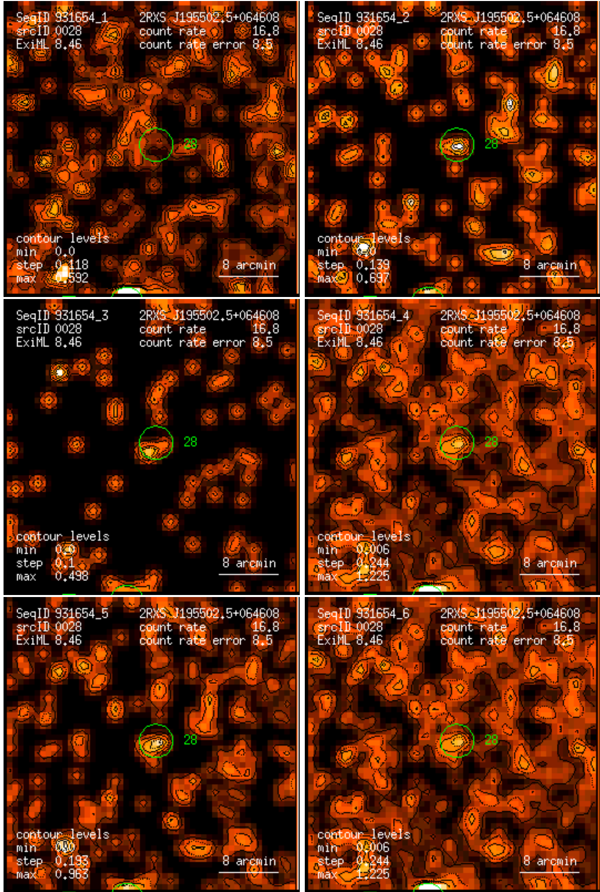
Figure 28: RASS 931654: detection 0028: band rate images, Gaussian filter: (1) PSPC channels 11 – 41, (2) 52 – 90, (3) 91 – 201, (4) 11 – 235, (5) 52 – 201, (6) 11 – 201. Broad band rates in counts/ks. Band rate contour levels in counts/ks/arcmin 2 .
