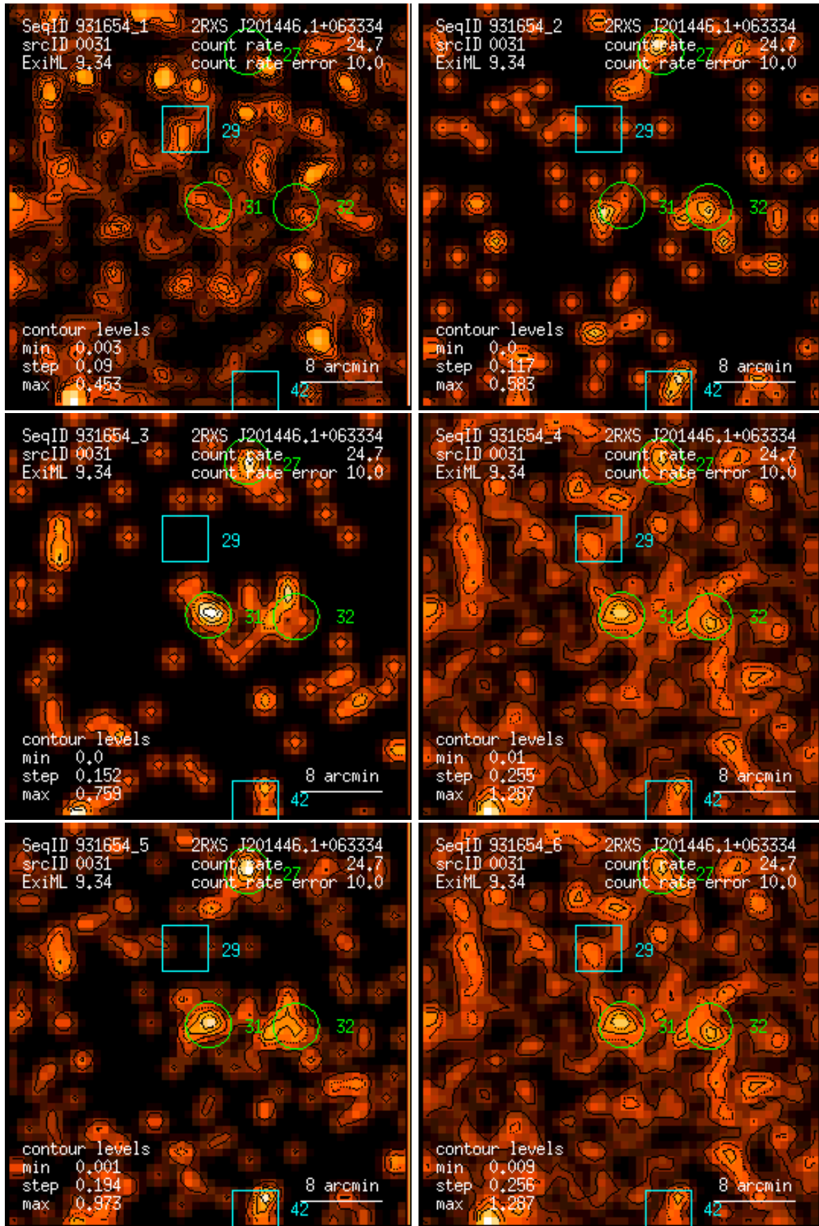
Figure 31: RASS 931654: detection 0031: band rate images, Gaussian filter: (1) PSPC channels 11 – 41, (2) 52 – 90, (3) 91 – 201, (4) 11 – 235, (5) 52 – 201, (6) 11 – 201. Broad band rates in counts/ks. Band rate contour levels in counts/ks/arcmin 2 .
