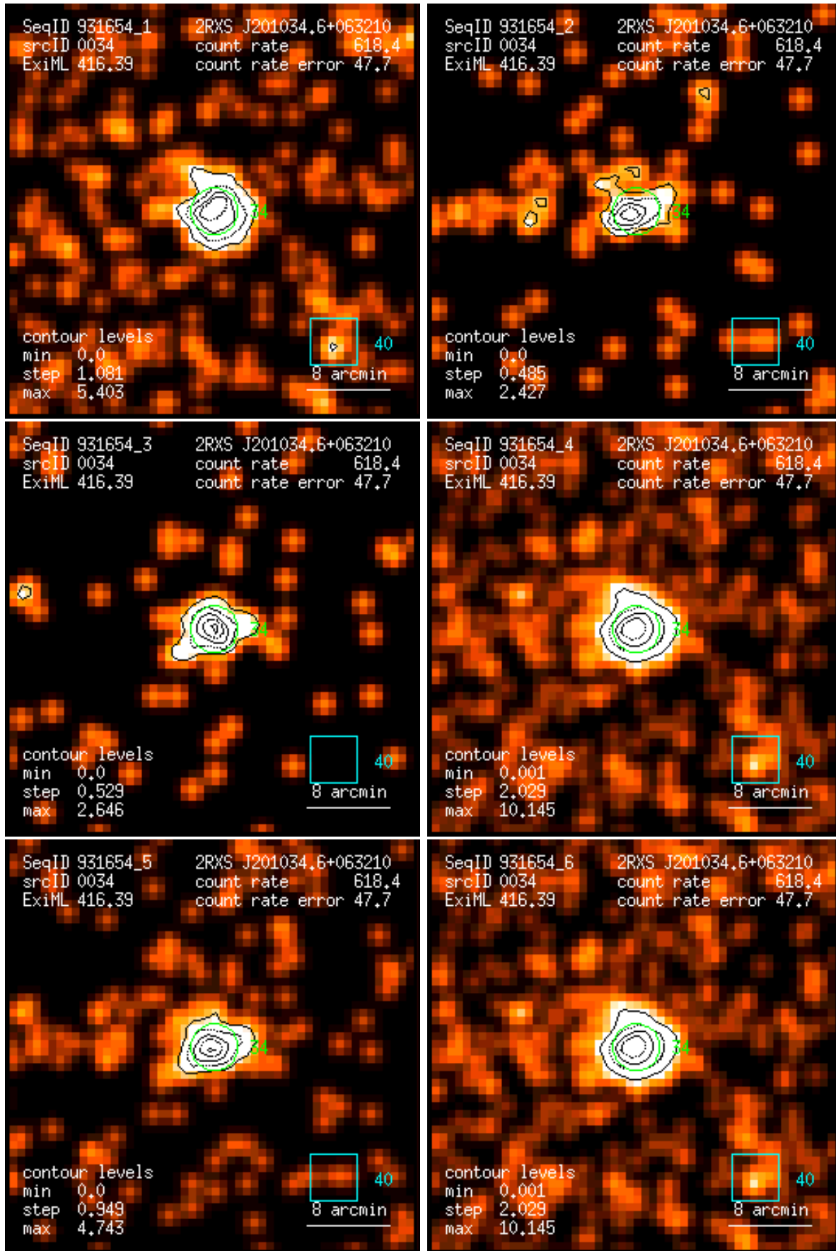
Figure 34: RASS 931654: detection 0034: band rate images, Gaussian filter: (1) PSPC channels 11 – 41, (2) 52 – 90, (3) 91 – 201, (4) 11 – 235, (5) 52 – 201, (6) 11 – 201. Broad band rates in counts/ks. Band rate contour levels in counts/ks/arcmin 2 .
