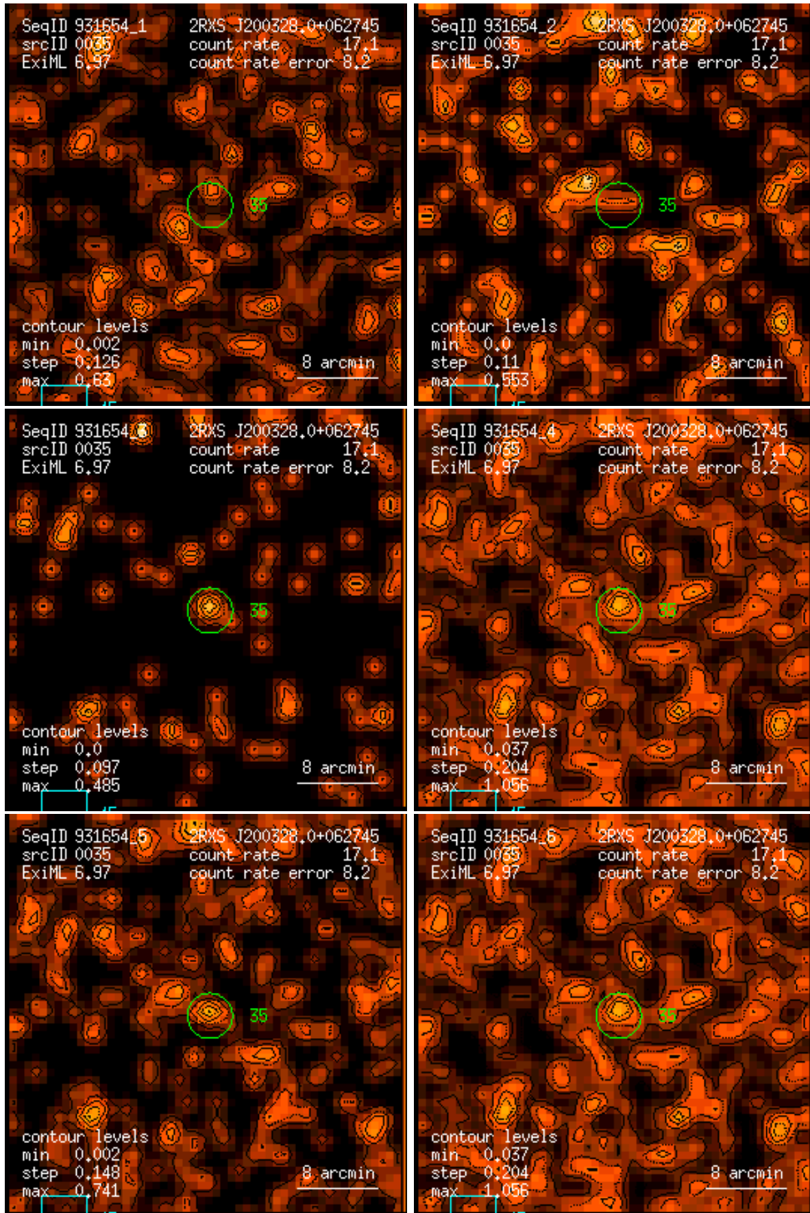
Figure 35: RASS 931654: detection 0035: band rate images, Gaussian filter: (1) PSPC channels 11 – 41, (2) 52 – 90, (3) 91 – 201, (4) 11 – 235, (5) 52 – 201, (6) 11 – 201. Broad band rates in counts/ks. Band rate contour levels in counts/ks/arcmin 2 .
