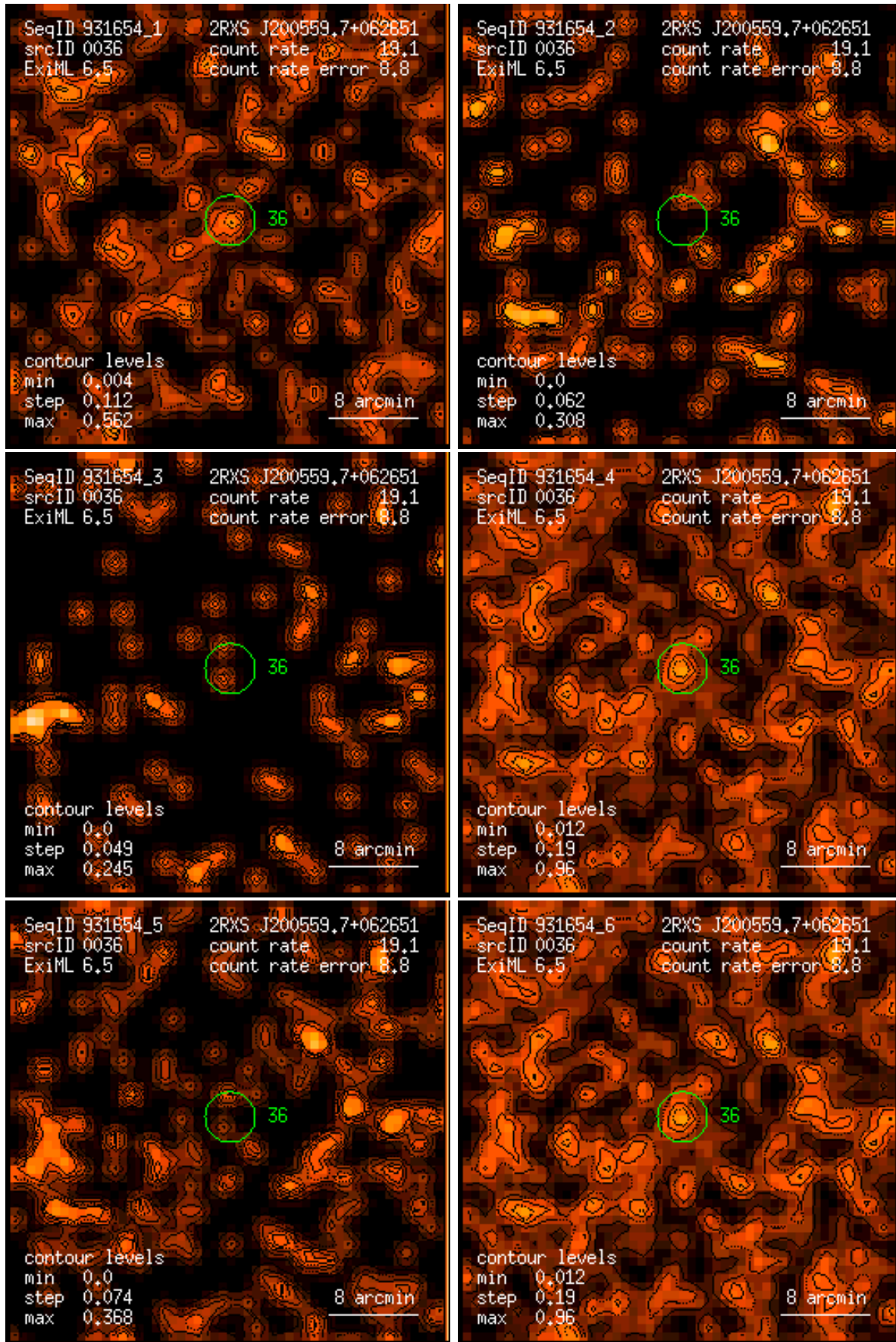
Figure 36: RASS 931654: detection 0036: band rate images, Gaussian filter: (1) PSPC channels 11 – 41, (2) 52 – 90, (3) 91 – 201, (4) 11 – 235, (5) 52 – 201, (6) 11 – 201. Broad band rates in counts/ks. Band rate contour levels in counts/ks/arcmin 2 .
