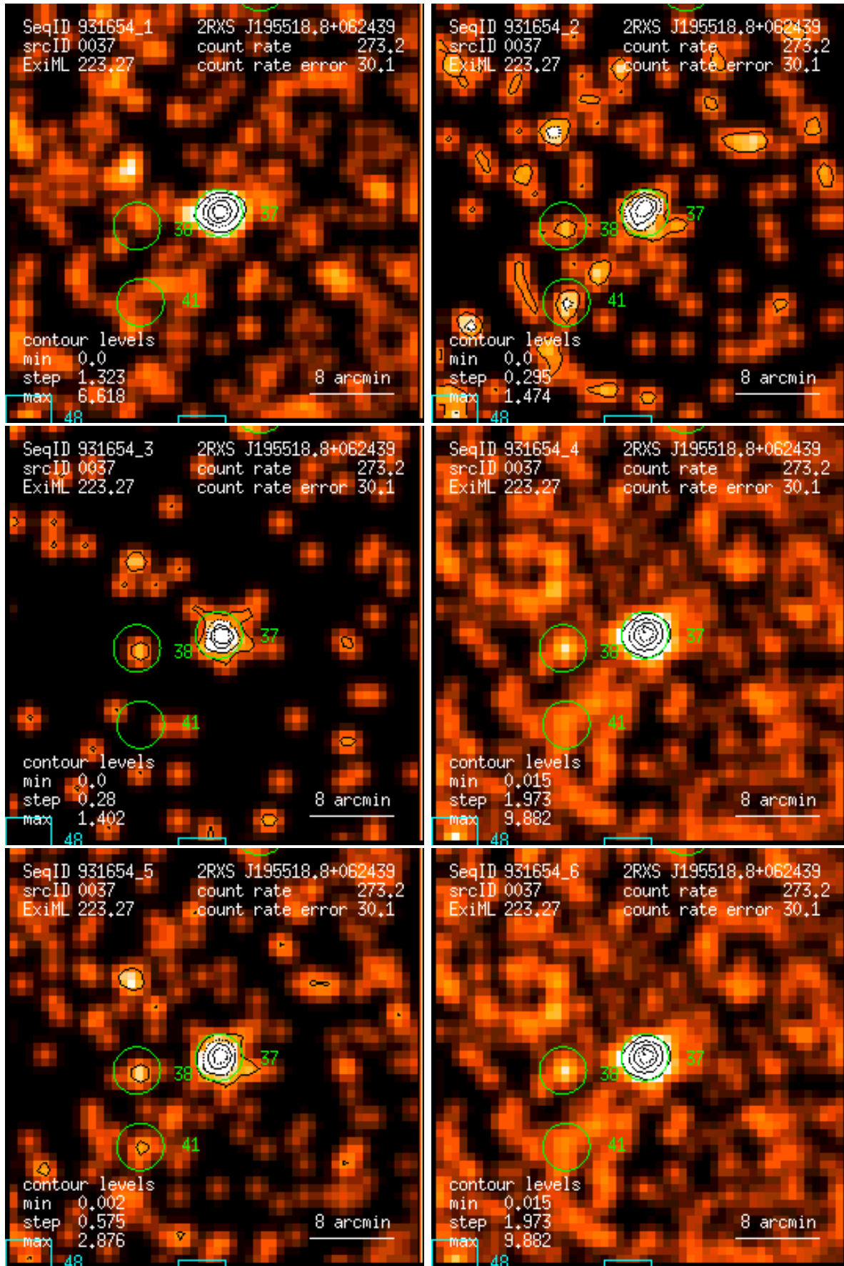
Figure 37: RASS 931654: detection 0037: band rate images, Gaussian filter: (1) PSPC channels 11 – 41, (2) 52 – 90, (3) 91 – 201, (4) 11 – 235, (5) 52 – 201, (6) 11 – 201. Broad band rates in counts/ks. Band rate contour levels in counts/ks/arcmin 2 .
