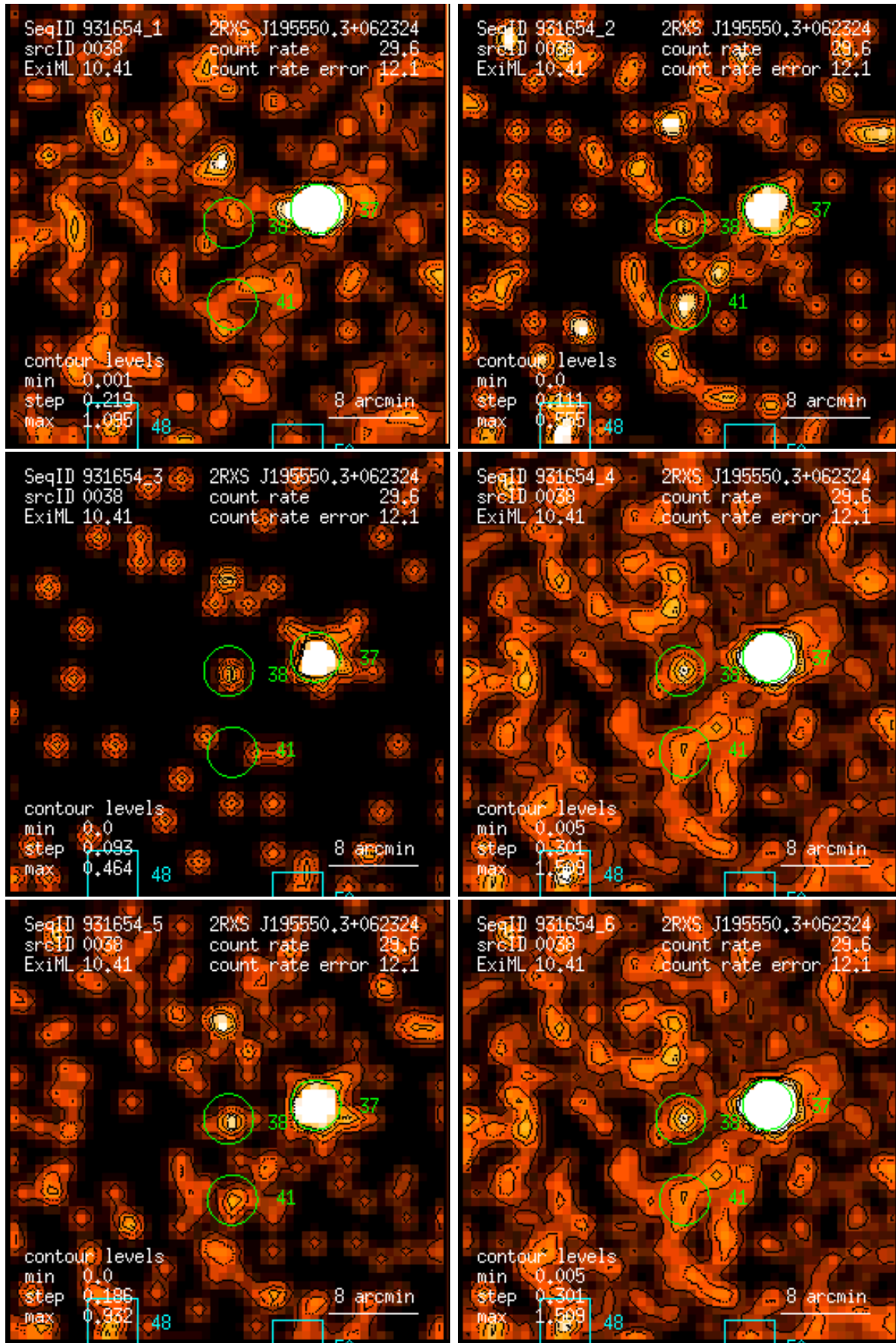
Figure 38: RASS 931654: detection 0038: band rate images, Gaussian filter: (1) PSPC channels 11 – 41, (2) 52 – 90, (3) 91 – 201, (4) 11 – 235, (5) 52 – 201, (6) 11 – 201. Broad band rates in counts/ks. Band rate contour levels in counts/ks/arcmin 2 .
