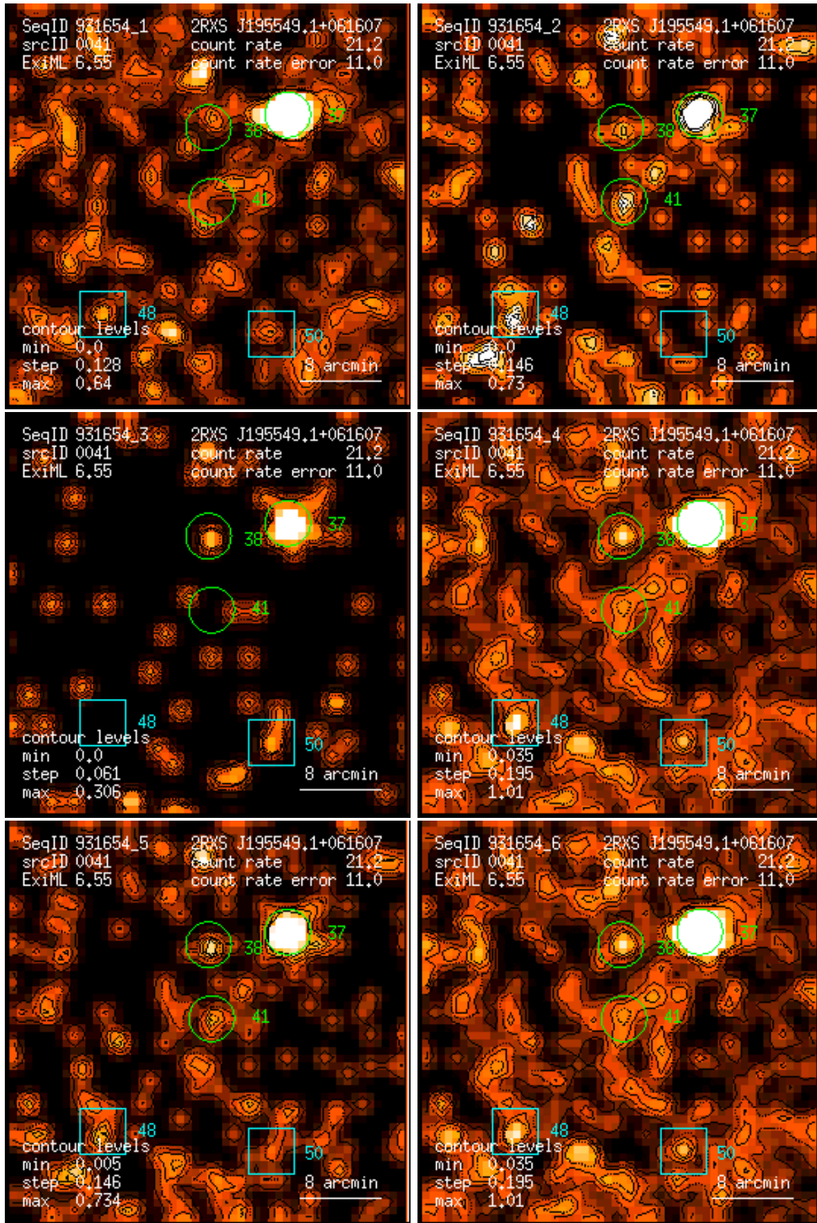
Figure 41: RASS 931654: detection 0041: band rate images, Gaussian filter: (1) PSPC channels 11 – 41, (2) 52 – 90, (3) 91 – 201, (4) 11 – 235, (5) 52 – 201, (6) 11 – 201. Broad band rates in counts/ks. Band rate contour levels in counts/ks/arcmin 2 .
