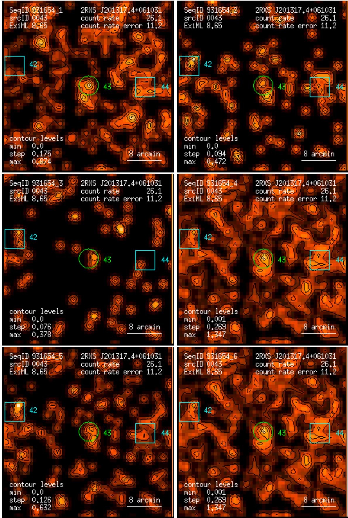
Figure 43: RASS 931654: detection 0043: band rate images, Gaussian filter: (1) PSPC channels 11 – 41, (2) 52 – 90, (3) 91 – 201, (4) 11 – 235, (5) 52 – 201, (6) 11 – 201. Broad band rates in counts/ks. Band rate contour levels in counts/ks/arcmin 2 .
